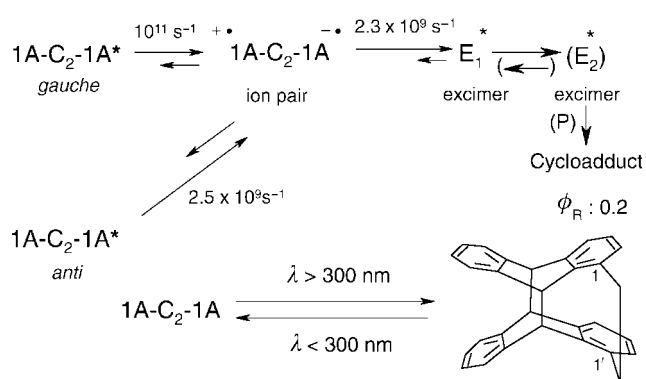
Scheme 12 Proposed reaction scheme for the photocycloisomerization of 1A-C_2-1A in acetonitrile . The two sets of conformers react at different rates and the ion pair was shown to collapse to excimer E_1^* which probably involves some harpooning effect. 29 For further details see Schemes 10 and 11. Possible back electron transfer from the ion pair to 1A-C_2-1A ground state has not been included in the Scheme.
