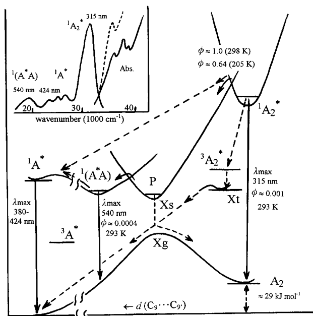
Fig. 13 Proposed energy profile for the photodissociation of the photodimers of dianthracene (A 2 ) and di(9-methylanthracene) (MeA) 2 in MTHF. At 293 K, the splitting occurs in the singlet state proceeding mainly through an electronically excited tight complex Xs (the pericyclic minimum) and partially through an excimer 1 (AA)*; the fluorescence quantum yields were found to be temperature dependent and very low at 293 K. At lower temperatures, the dissociation was shown to follow the triplet ( 3 A 2 *) route which is exclusive at 77 K. Insert: absorption and uncorrected fluorescence spectra of a degassed 10 -4 M solution of A 2 in MTHF at 293 K (λ exc. 270 nm). Adapted from Yamamoto and Grellmann, 30 with permission.
