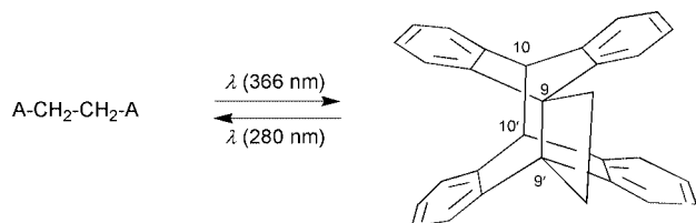
Scheme 10 Photocycloisomerisation of 1,2-di(9-anthryl)ethane ( A-CH_2CH_2-A ) in MCH:IP ; excimer ( E_2^* ), characterized at 77 K, was not observed at ambient temperature presumably because the fluorescence cannot compete with the photoreaction. The 'monomer' is a mixture of ground state conformers. (P) denotes the pericyclic minimum (see Fig. 6).
