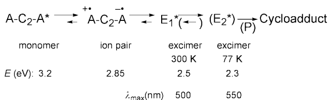
Scheme 11 Possible reaction scheme for 1,2-di(9-anthryl)ethane ( AC_2A ) photocycloisomerization in acetonitrile at ambient temperature. Excimer ( E_2^* ) was characterized only at low temperature (Hayashi et al. 1976, 28 ). The ion pair was detected by ps flash photolysis (Yao et al. 28 ). E (eV) \equiv excited state energy. For other symbols see Scheme 10.
