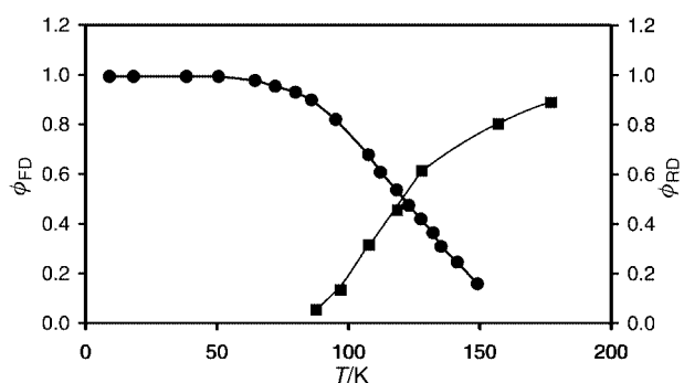
Fig. 4 Temperature dependence of the photodimerization ( \phi_{\text{RD}} ) and excimer fluorescence ( \phi_{\text{FD}} ) quantum yields of the anthracene sandwich pair in dianthracene matrix. Taken from Ferguson and Mau 1974 8–10 with permission.
