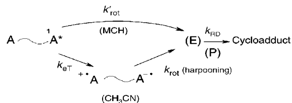
Scheme 13 Suggested mechanism for photocycloaddition of ACH_2OCH_2A or AOCH_2OA in non polar ( MCH ) or polar ( CH_3CN , CH_3OH ) solvents; k_{rot} , k'_{rot} denote bond rotation rate constants to attain a non fluorescent excimer (E) geometry; eT denotes electron transfer. It is assumed that k_{RD} \gg k_{rot} and k'_{rot} .
