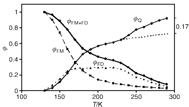
Fig. 5 Temperature variation of the fluorescence quantum yields ( \phi ) of ASiMe 2 OSiMe 2 A in a degassed mixture of methylcyclohexane (MCH) and isopentane (IP). MCH:IP = 1:3. FM = monomer fluorescence; FD = excimer fluorescence; Q = quenching. \phi_Q = 1 - \phi_{FM+FD} . Taken from ref. 16 with permission.
