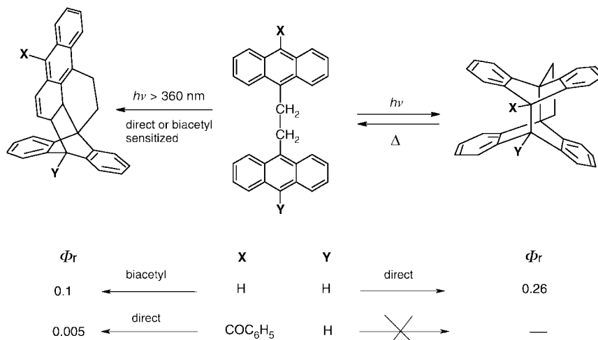
Fig. 11 Direct and triplet sensitized (typically AC 2 A 2 \times 10^{-3} M in benzene at 420 nm, with biacetyl 2 \times 10^{-1} M under argon) irradiation of di(9-anthryl)ethane derivatives. The phosphorescence of biacetyl has been found to be quenched at nearly diffusion controlled rate.
