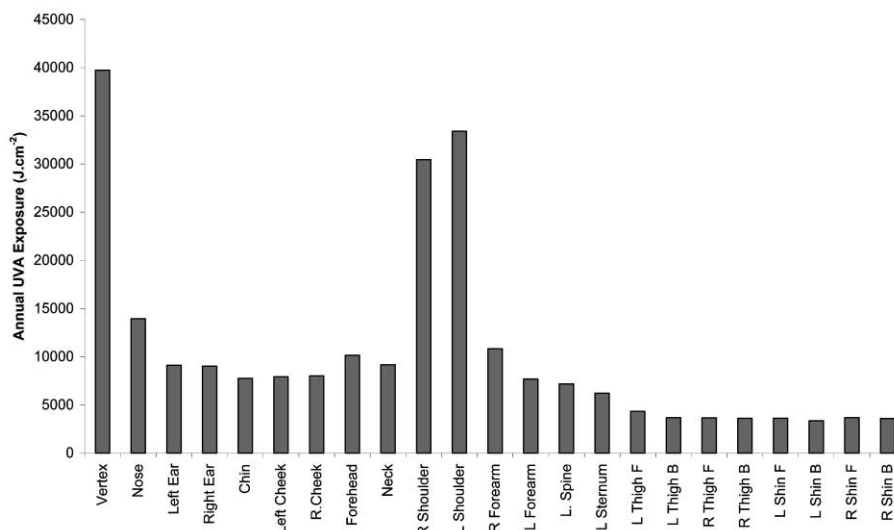
Fig. 3 The annual UVA exposure to various anatomical sites for a person in an upright position.
