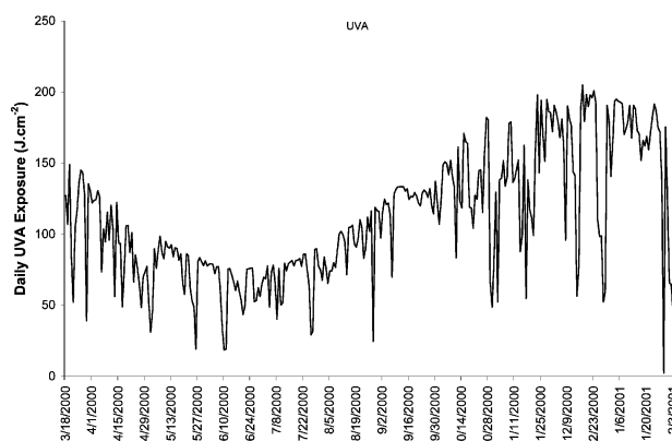
Fig. 1 The measured UVA exposures on a horizontal plane.
