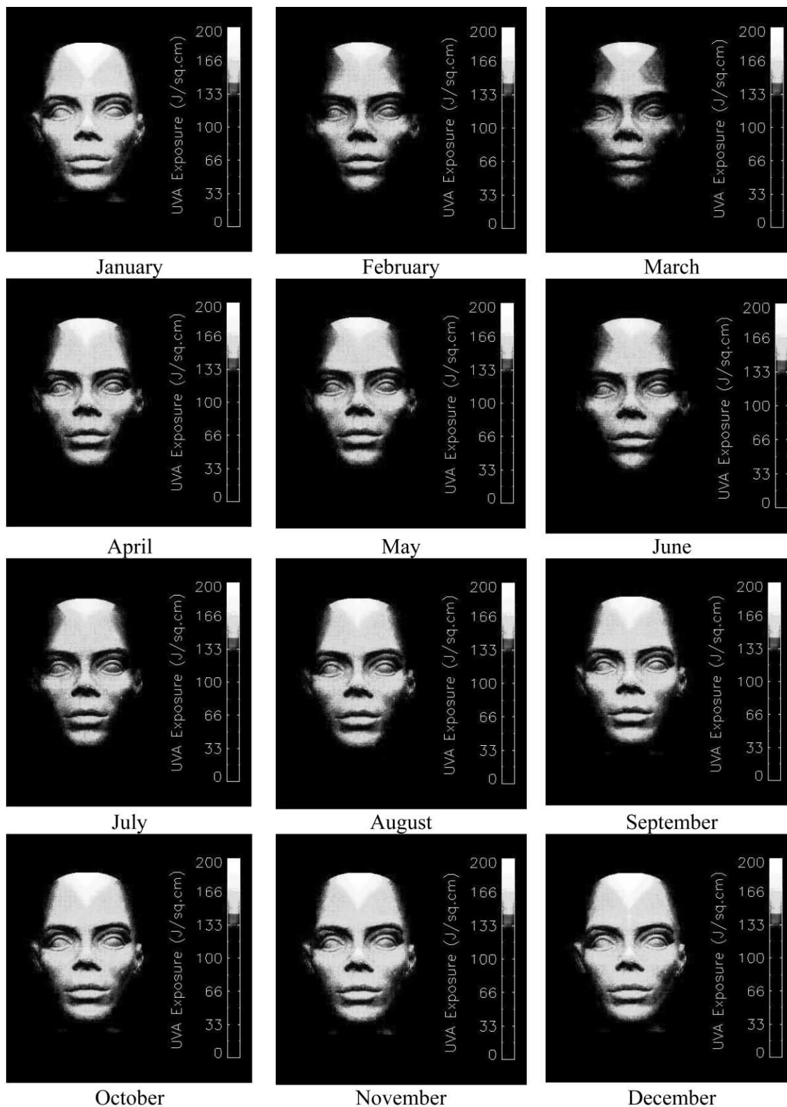
Fig. 4 The facial distribution of UVA exposure over the period of one year.
