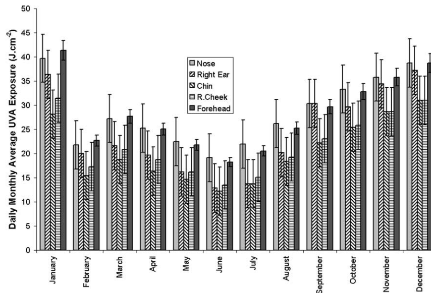
Fig. 2 The daily UVA exposures averaged over each month for various anatomical locations.
