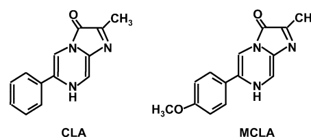
Fig. 1 Structures of CL probes, CLA and MCLA.
