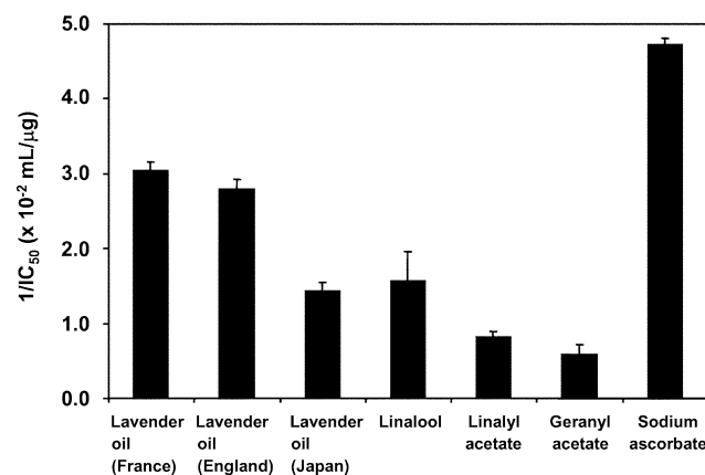
Fig. 7 Singlet oxygen ( ^1\text{O}_2 ) quenching activity in terms of 1/\text{IC}_{50} value of lavender oils and their major components, compared with sodium ascorbate. \text{IC}_{50} value was defined as 50% inhibitory concentration of the materials for the generated ^1\text{O}_2 in the hematoporphyrin–UVA system.
