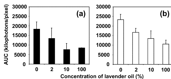
Fig. 8 Suppressive effect of a lavender oil made in France on CL intensity attributable to ROS generation in both the intact and UVA-exposed skin of live mice in terms of AUC values for 0–30 min of CL measurement. Lavender oil suppressed dose-dependently at the concentrations of 2, 10 and 100% both intrinsic (a) and UVA-induced (b) ROS generation. Data are expressed as means \pm standard deviations ( n = 3–5 ).
