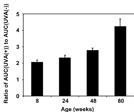
Fig. 5 Age-dependent enhancement of the ratio of CL intensities attributable to ROS generation in UVA-exposed skin to those in the untreated skin of hairless rats aged 8, 24, 48, and 80 weeks. CL intensities due to ROS generation in the skin of the untreated and UVA-exposed ( 20 \text{ mW cm}^{-2} \times 5 \text{ min} ) rats at 8, 24, 48, and 80 weeks old were measured, and AUC values for the CL levels were calculated from the time-dependent curves, and then the ratio of AUC [UVA (+)] to AUC [UVA (-)] was calculated in the rats at the corresponding age. Data are expressed as means \pm standard deviations ( n = 6 ).
