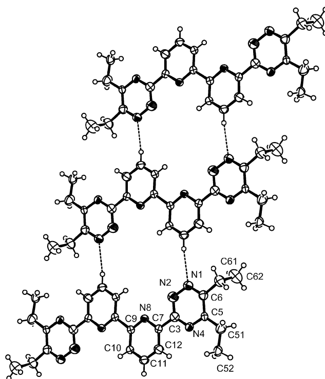
Fig. 4 The structure of C2-BTBP, which has the etc conformation, with ellipsoids at 25% probability showing how the molecules pack in the c direction. Intermolecular hydrogen bonds are shown as dotted lines.
