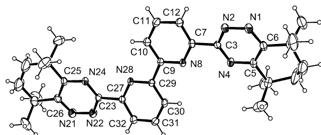
Fig. 5 The structure of \text{CyMe}_4 -BTBP, which has the ttt conformation, with ellipsoids at 25% probability.
