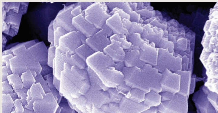
Novel drum-like Cd(OH) 2 superstructures synthesised by Fen Gao and Qingyi Lu's laboratory, Nanjing University, P R China, on a large scale through a facile one-pot hydrothermal route with the co-existence of ammonia and biopolymer sodium carboxymethyl cellulose solutions ( Chem. Commun. , 2011, 47 , 4141)
