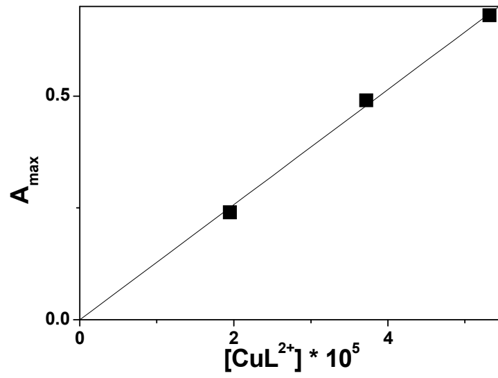
Fig. S1. Absorbance ( A_{\text{max}} ) at the maximum of the band at \sim 400 nm of \text{CuL}^{2+} in DNA, \text{CuL}^{2+} , \text{W/C}_{12}\text{E}_4 systems as function of complex concentration.
