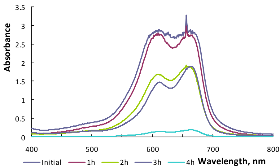
Figure S1. UV plot for the visible light photobleaching of methylene blue over N -doped nano TiO 2 .
