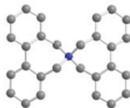
NMR enantiodifferentiation
