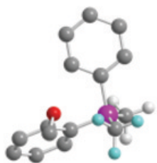
NMR enantiodifferentiation
