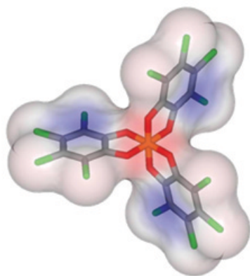
NMR enantiodifferentiation
