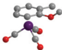
NMR enantiodifferentiation
