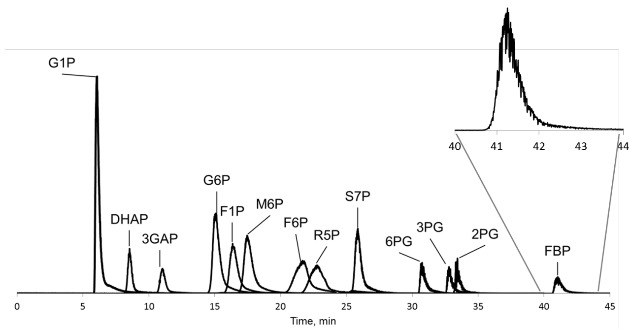
ESI 3 Chromatogram of 50 \mu M standard solutions of sugar phosphates obtained employing AEC in combinations with online post column ion suppression.
