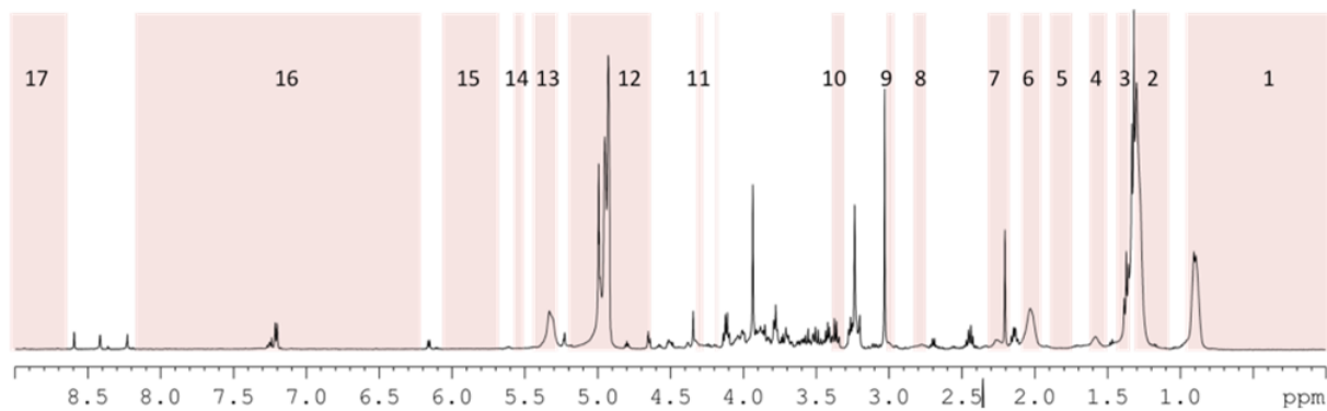
Fig. S1: Muscle spectrum example, with the excluded regions in color, labelled according to Table S1.
