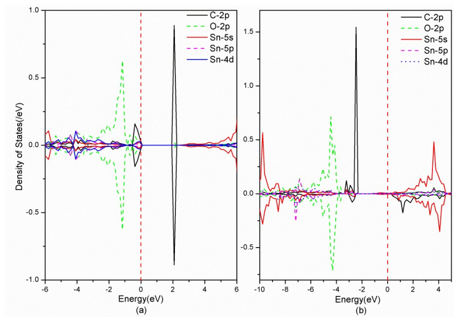
Figure S1. HSE06 function calculated PDOS of C_O defects in (a) neutral and (b) -2 charge state, respectively. The vertical red dashed line represents Fermi level.
