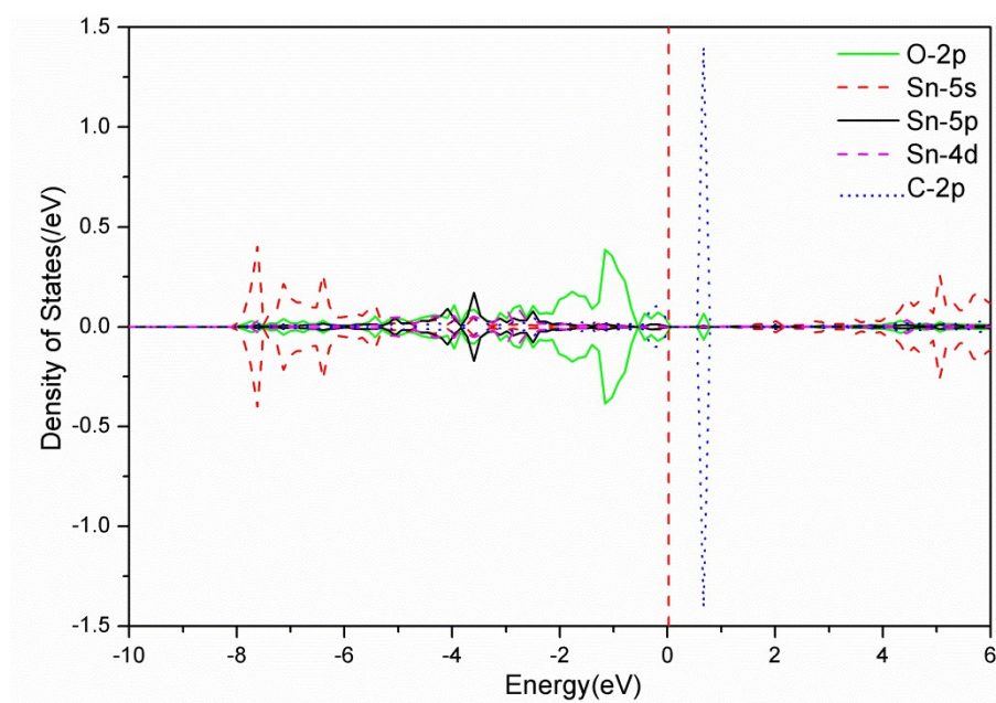
Figure S2. PDOS of bulk SnO 2 :C materials calculated by GGA function. The vertical red dashed line represents Fermi level.
