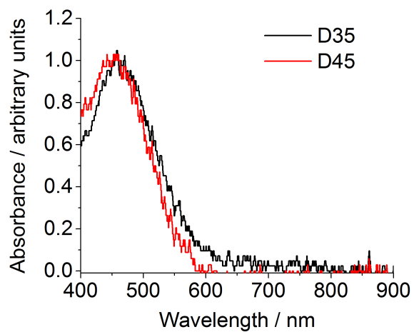
Figure S1. Absorbance of the organic dyes D35 and D45 sensitized on spin coated TiO 2 films.
