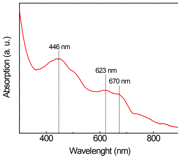
Figure S2 UV-Vis spectra of single layer Ex-MoS 2 dispersion in H 2 O.
