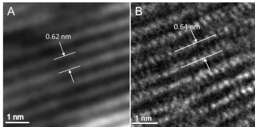
Figure S1 HRTEM images show the cross-sectional view of (A) bulk-MoS 2 and (B) Ex-MoS 2 along the c -axis.
