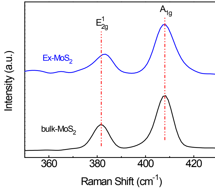
Figure S3 Raman spectra of bulk MoS 2 and ex-MoS 2 of E 2g 1 and A 1g peaks.
