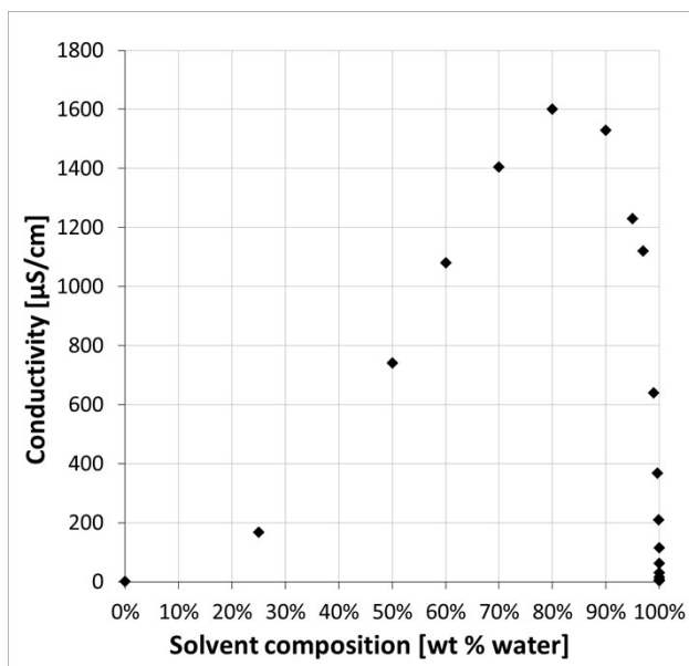
Figure S1: Electrical conductivity of acetic acid–water mixtures. 29
