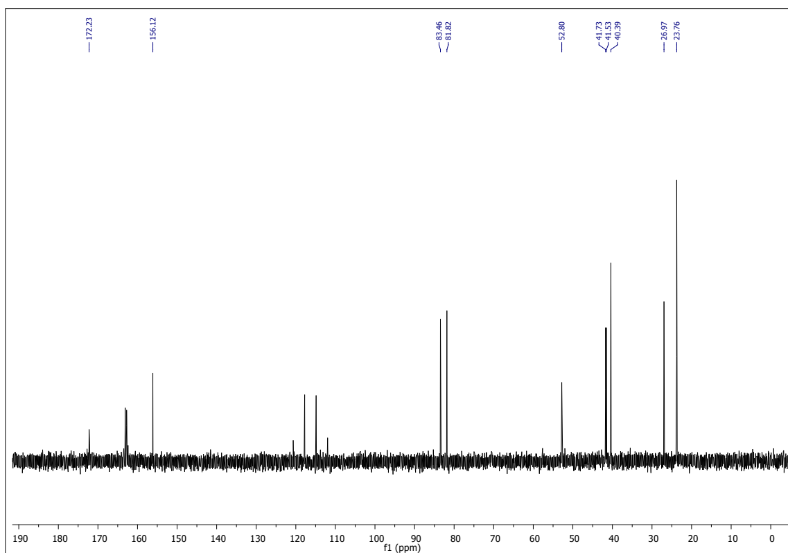
13 C NMR Compound 6d
