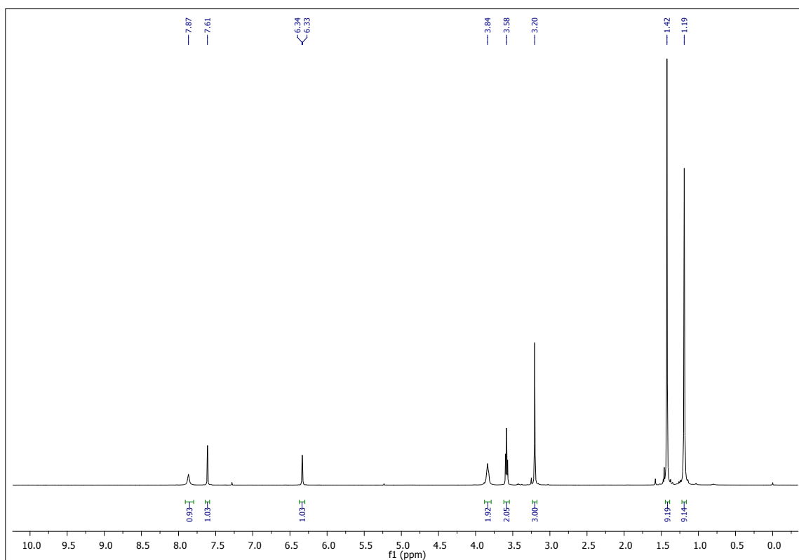
1 H NMR Compound 3f
