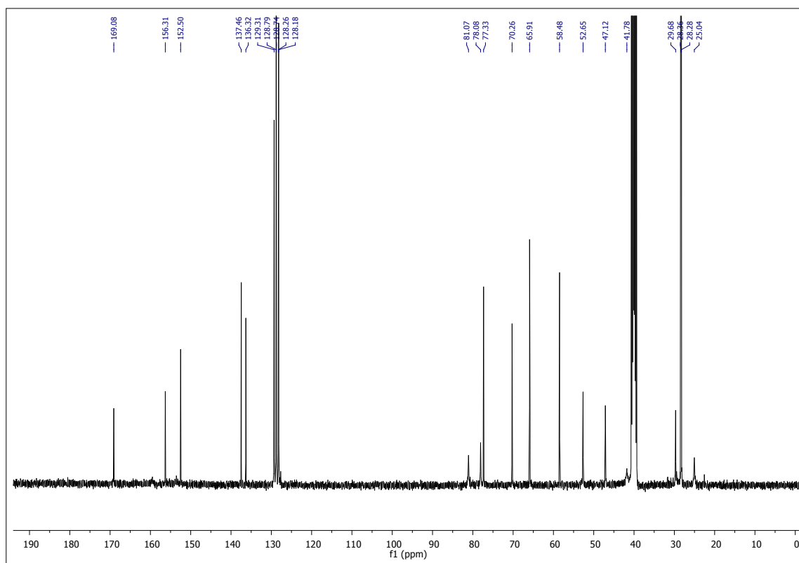
13 C NMR Compound 9c
