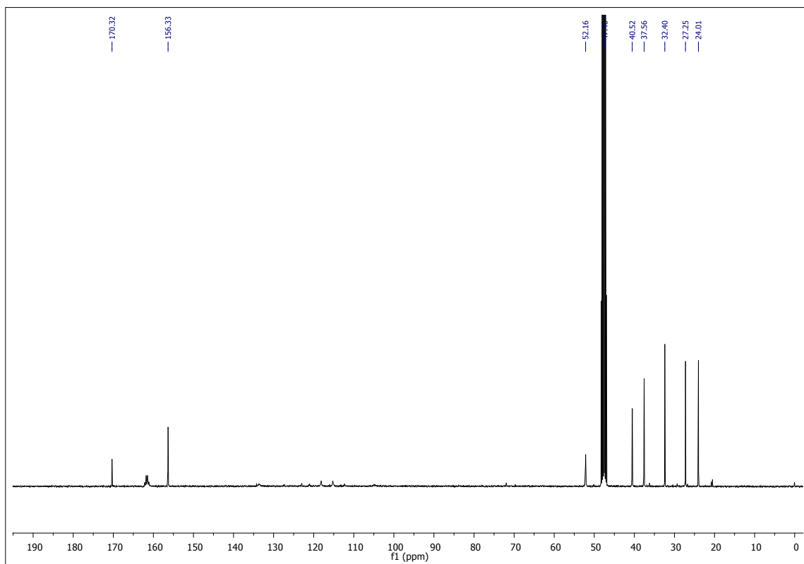
13 C NMR Compound 6a
