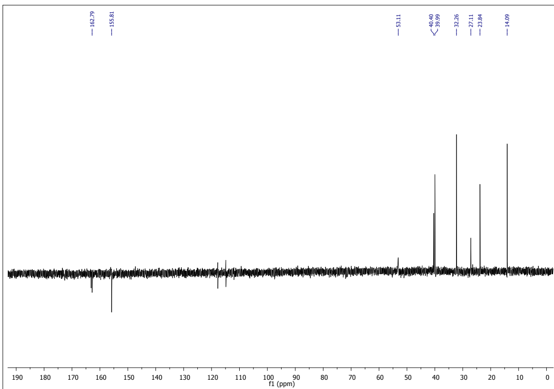
13 C NMR Compound 6c
