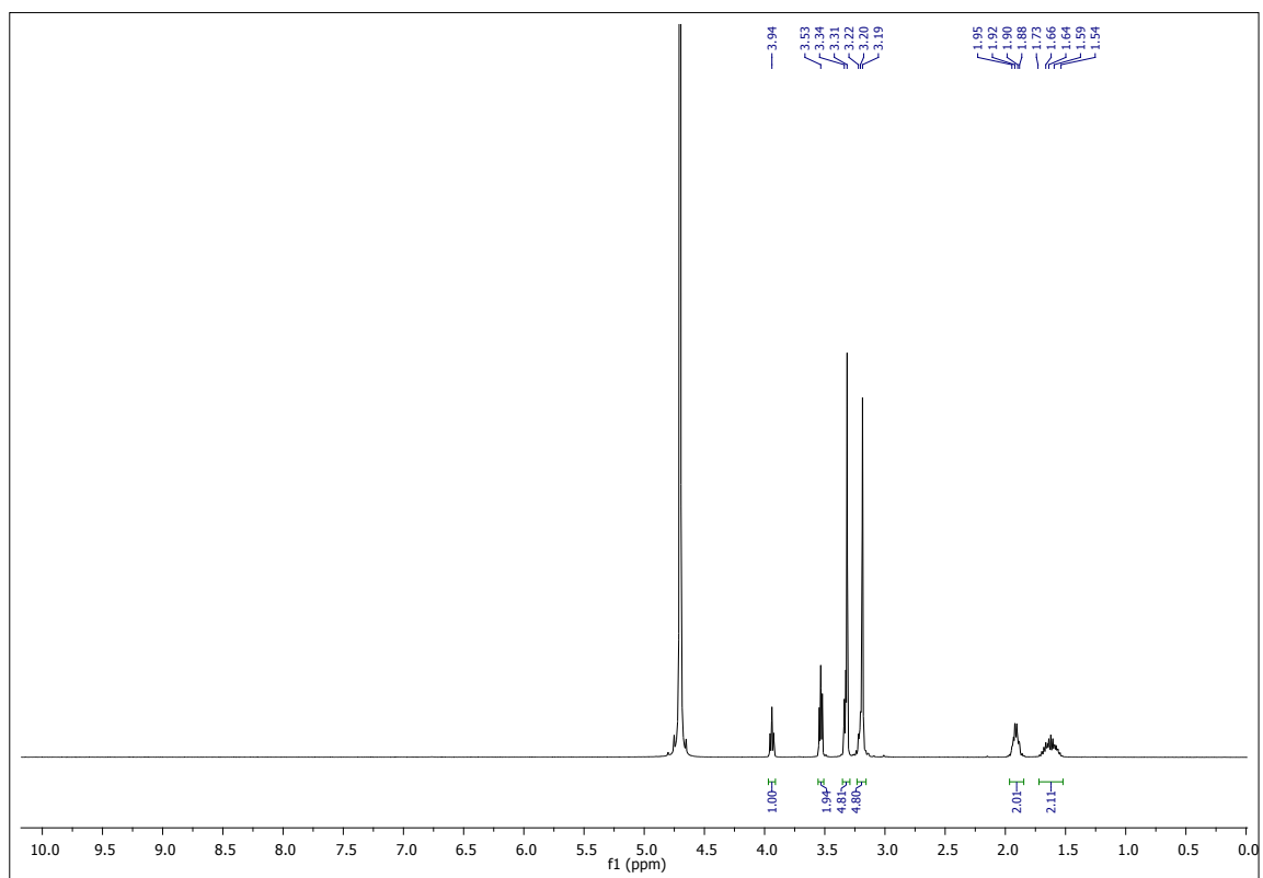
1 H NMR Compound 10a
