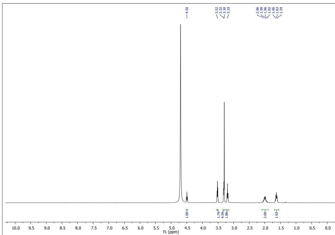
^1\text{H} NMR Compound 14b
