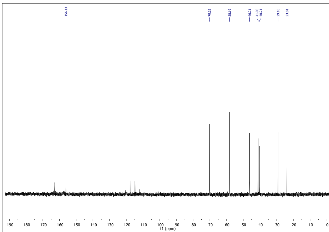
^{13}\text{C} NMR Compound 14a
