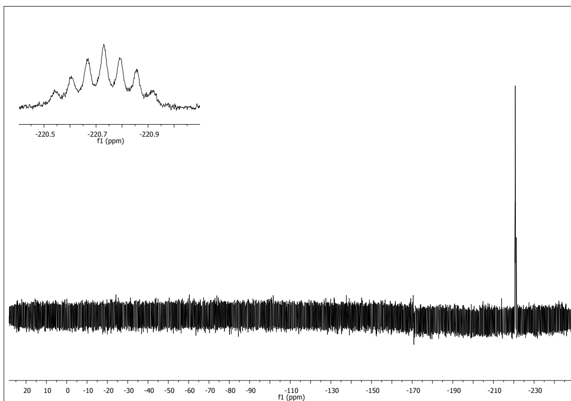
^{19}\text{F} NMR Compound 5d
