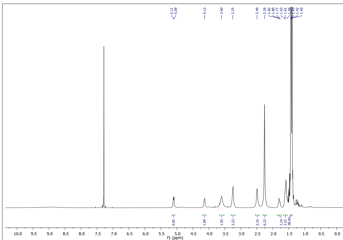
1 H NMR Compound 5b
