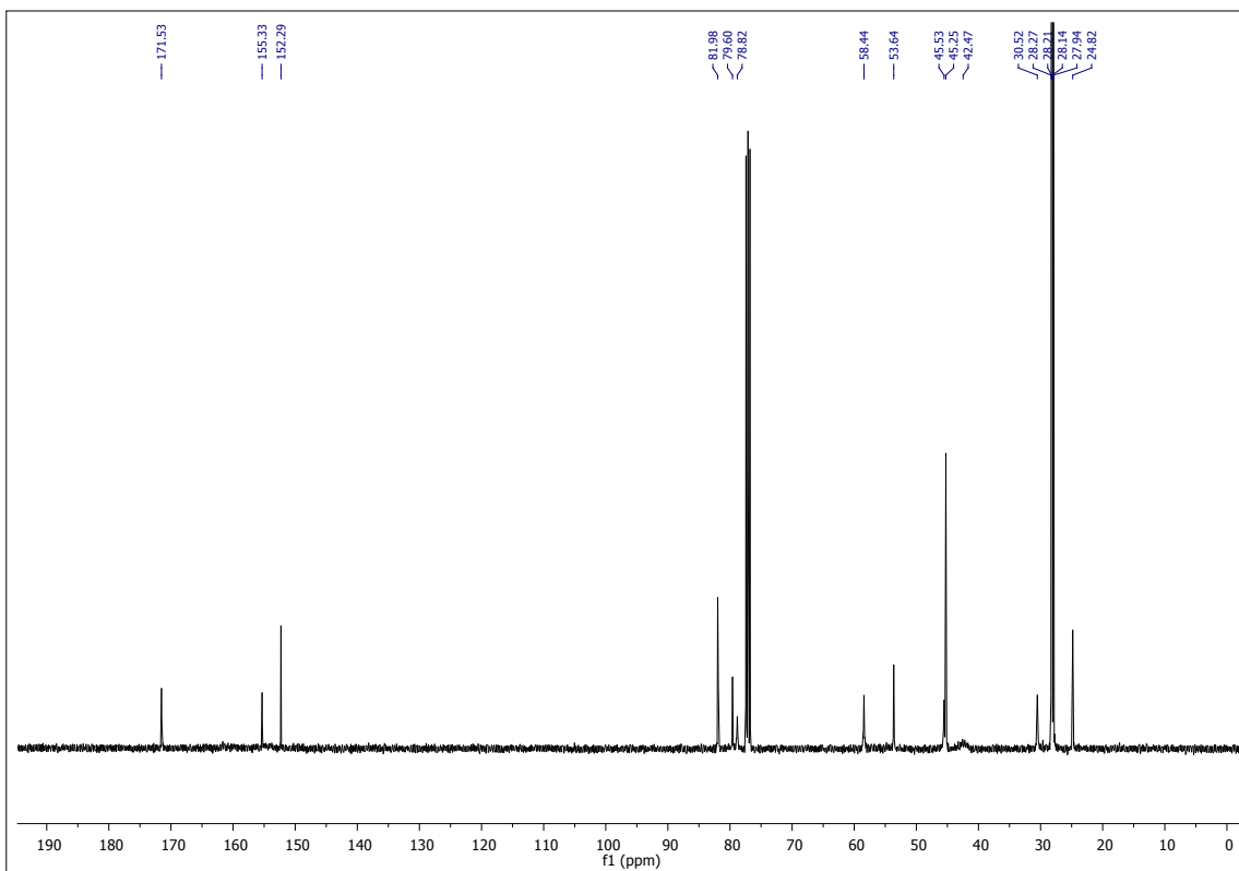
1 H NMR Compound 5c
