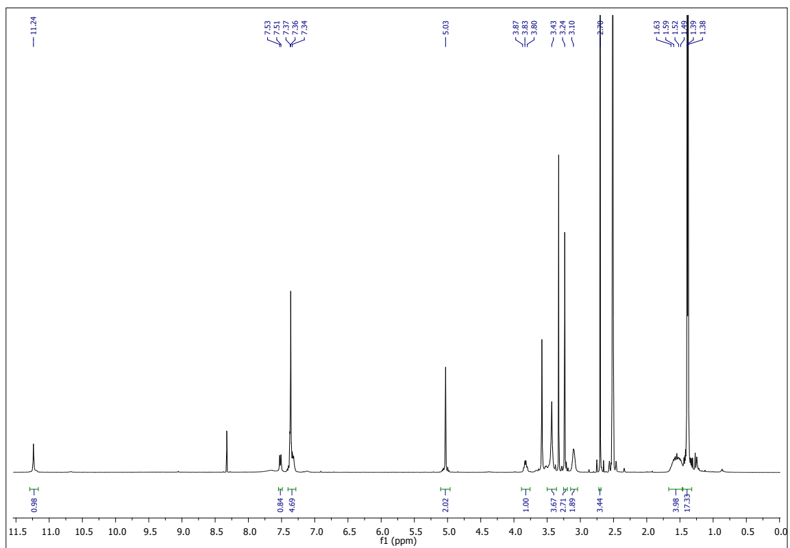
1 H NMR Compound 9b
