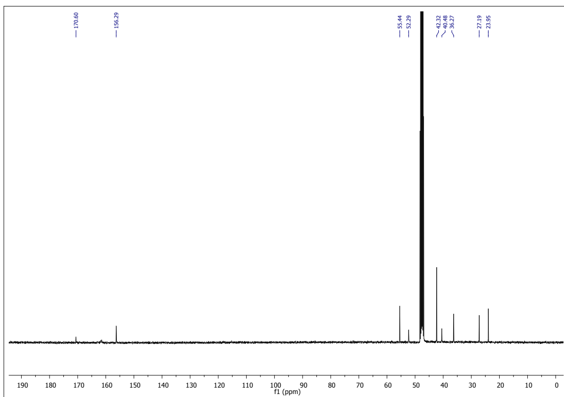
13 C NMR Compound 6b
