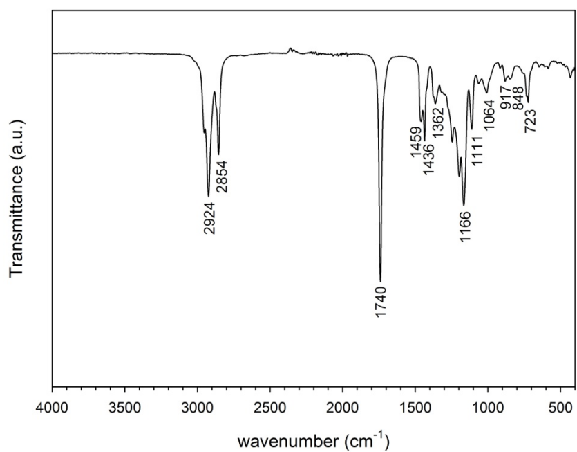
Figure S2. IR spectrum of product of Friedel-Craft reaction of decanoic acid
