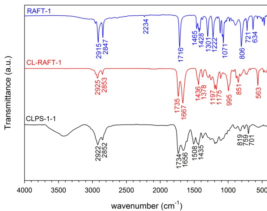
Figure S1. IR spectrum of CL-RAFT-1, compared to that of RAFT-1 and CLPS-1-1
