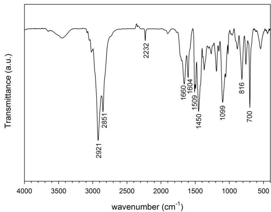
Figure S3. IR spectrum of CLPS 4-1
