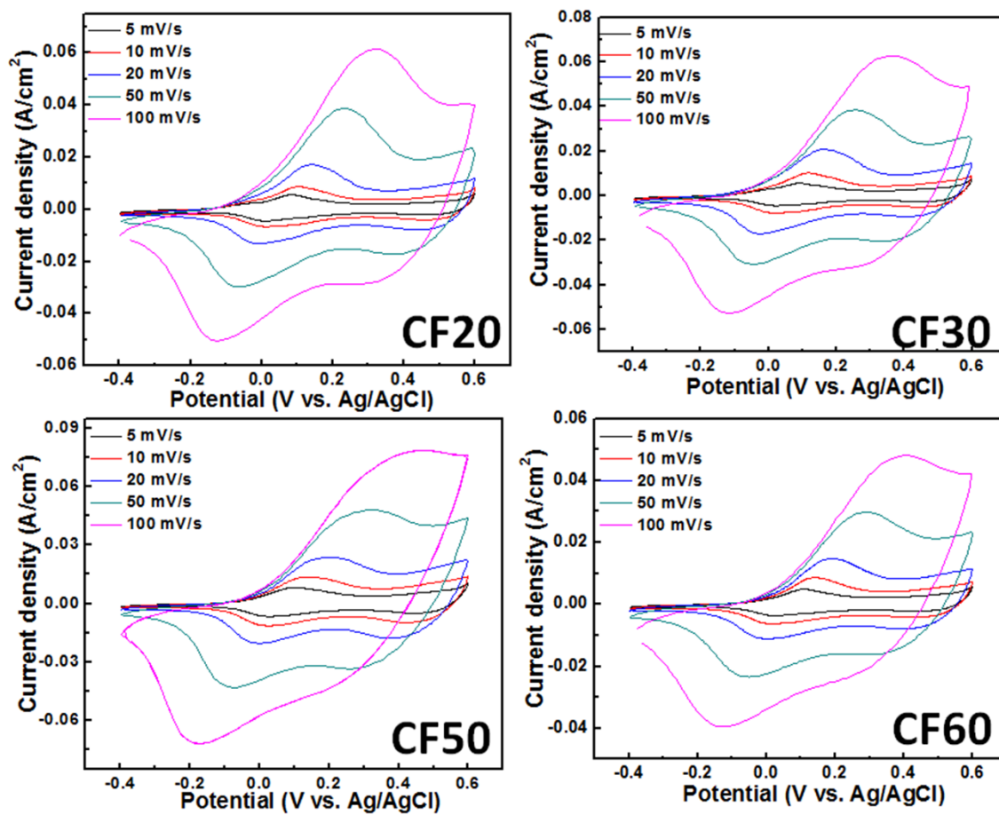
Fig. S1 CV curves of CF20 CF30 CF50 and CF60 electrodes at scan rates of 5, 10, 20, 50 and 100 mV/s;
