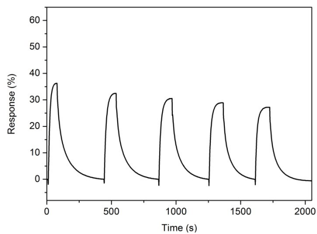
Fig. S2 The reproducibility of temporal response of ZnO-rGO-Au hybrids exposed to 100 ppm NO 2 80 °C.
