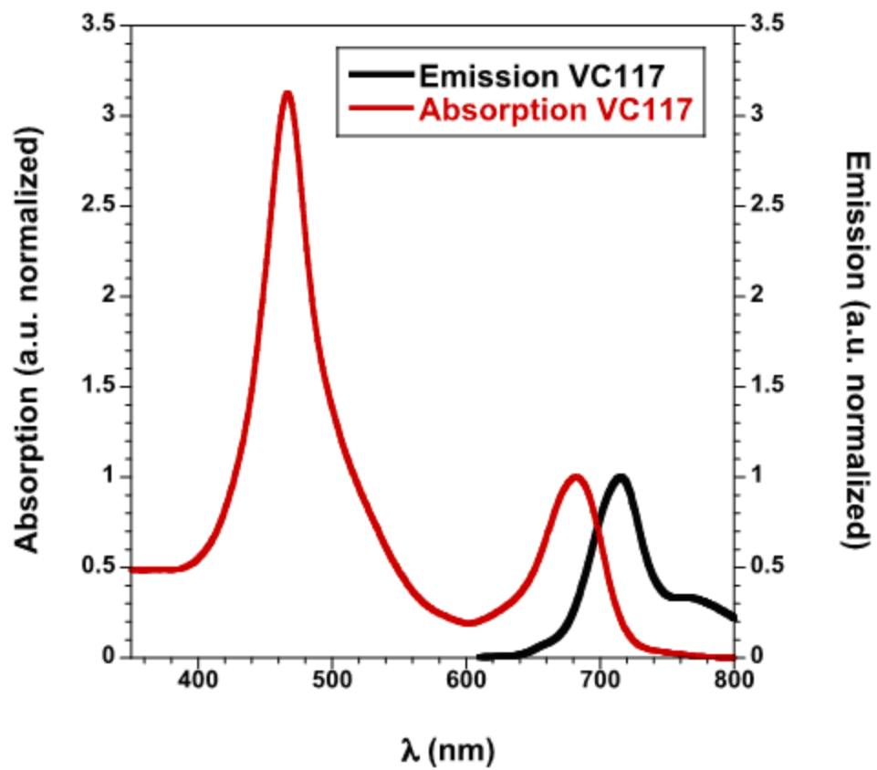
Figure S7 Normalized absorption and emission spectra of VC117 in solution.
