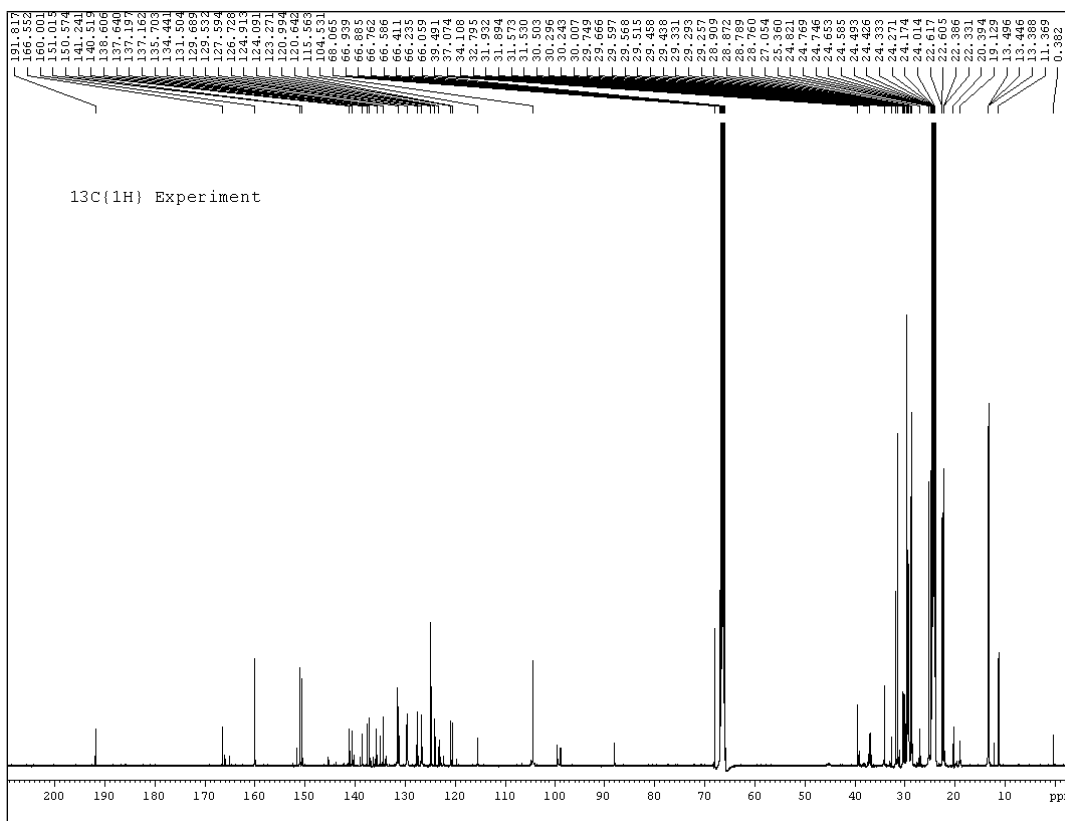
Fig. S5 13 C NMR spectra of compound VC117 recorded in THF-d 8 .
