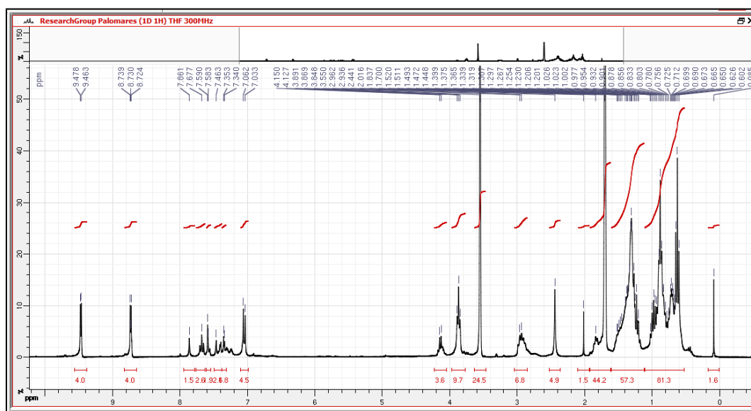
Fig. S4 ^1\text{H} NMR spectra of compound VC117 recorded in THF-d 8 .
