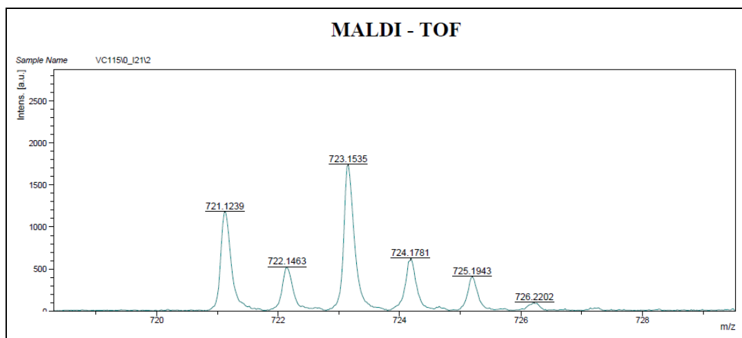
Fig. S3 MALDI-TOF spectra of compound 3.
