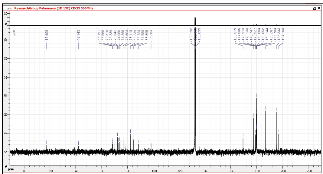
Fig. S2 ^{13}\text{C} NMR spectra of compound 3 recorded in \text{CDCl}_3 .
