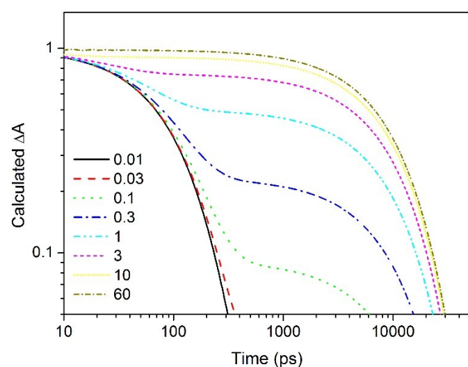
Figure S1. Numerically calculated TAS kinetics for the time range from 10 ps up to 60 ns. Used data set was the same as that used in Figure 11.
