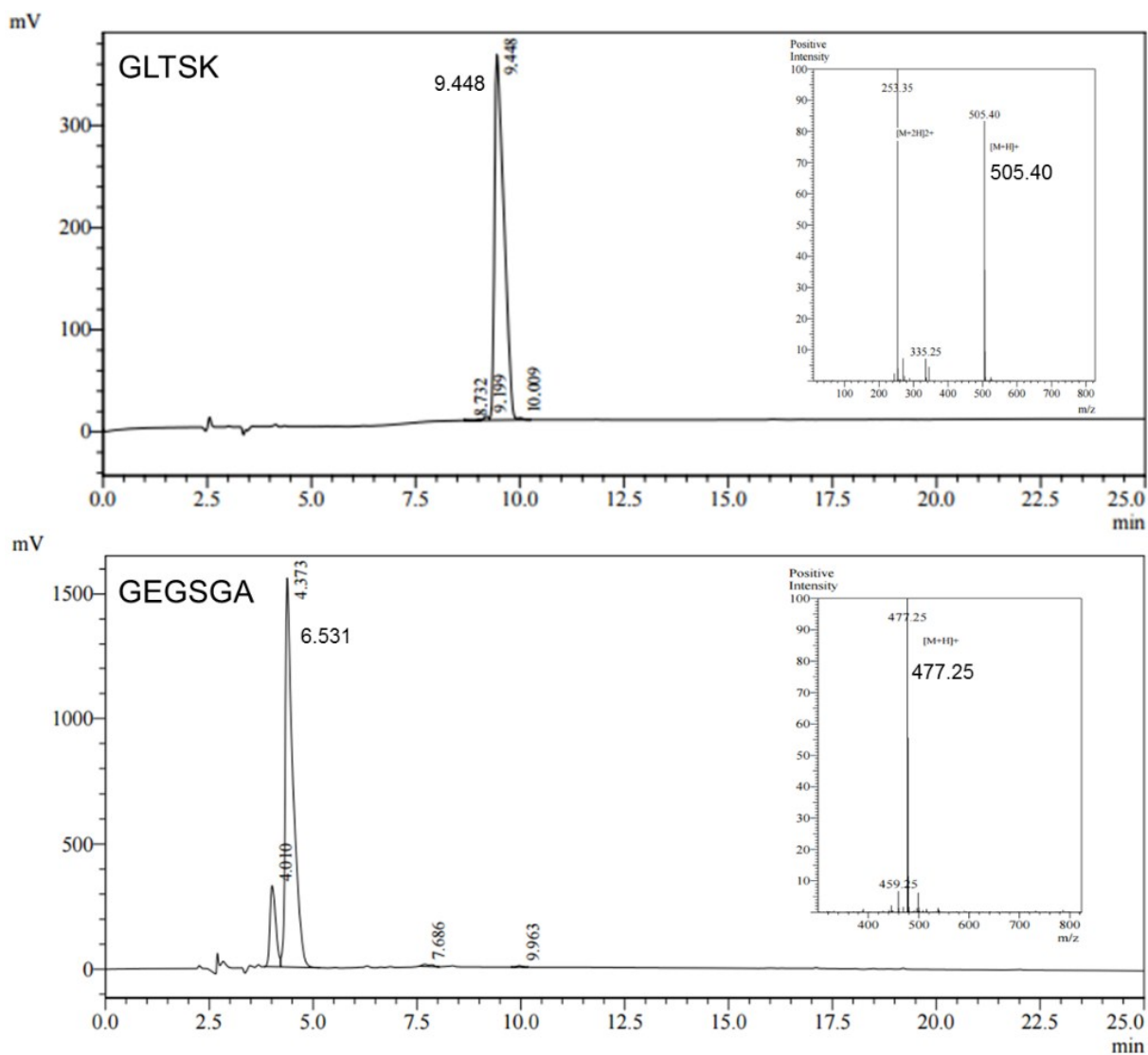
Supplemental Figure 1: Chromatograms (left) and mass/mass spectra (right) of pure peptides originally found in NDF of common bean.
