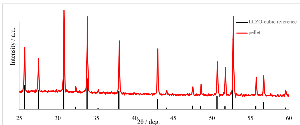
Figure S1: XRD of sol-gel synthesized pellet
