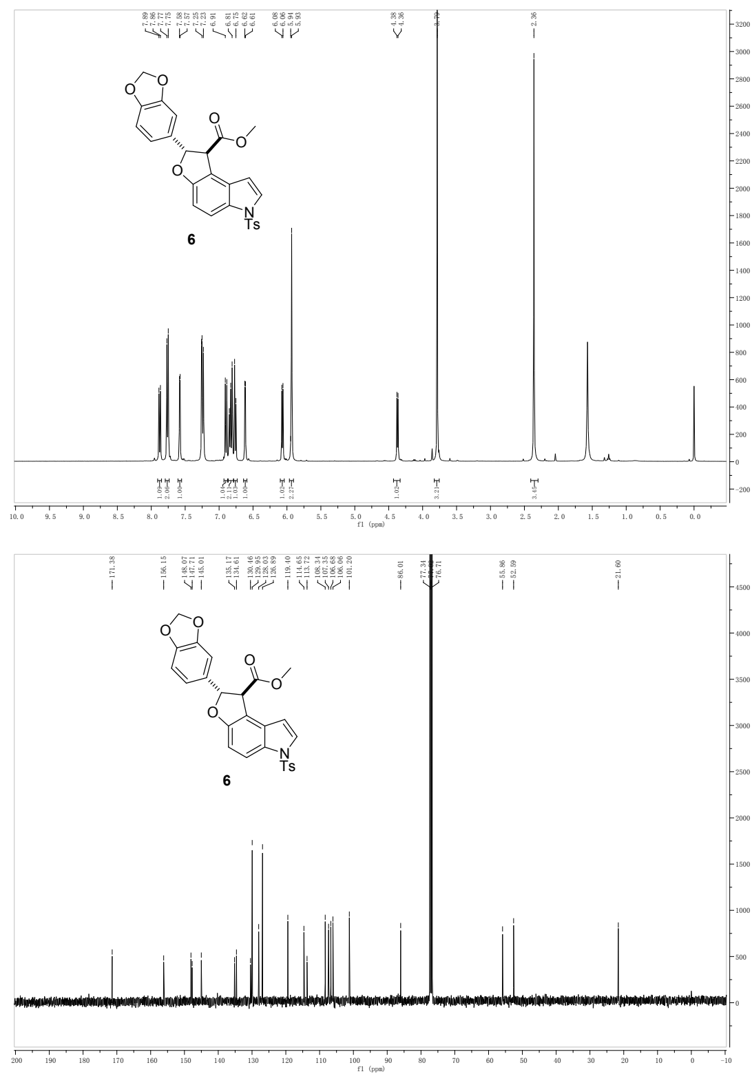
Figure S1. Copies of ^1\text{H} NMR and ^{13}\text{C} NMR spectra
