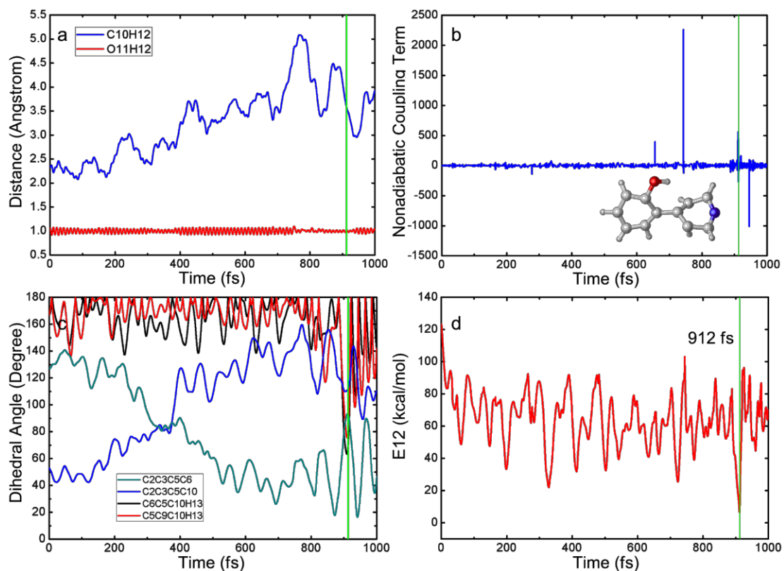
Fig. S4: Time-dependent physical variables of two other typical OM2/MRCI trajectories involved (I) S1-ENOL and S1S0-ENOL-1 and (II) S1-ENOL and S1S0-ENOL-2: (a) two key bond lengths; (b) nonadiabatic coupling term; (c) four key dihedral angles; and (d) S 1 -S 0 energy gap.
