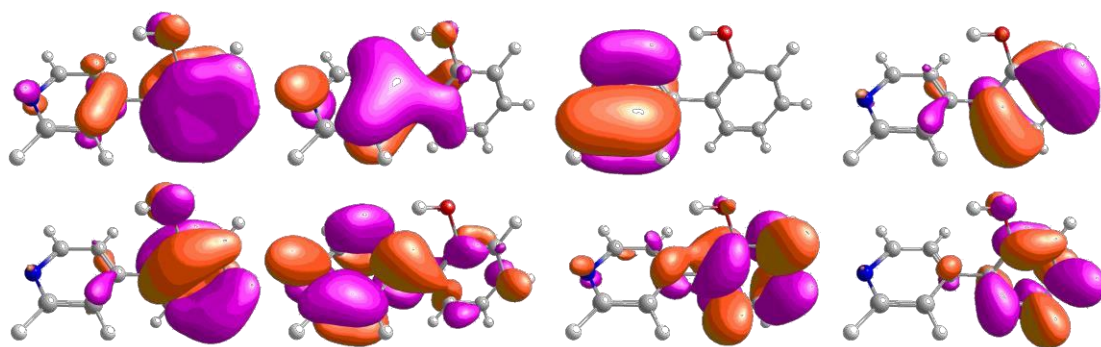
Fig. S1: Natural molecular orbitals used for the active space of CASSCF and CASPT2 methods. See main text for discussion.
