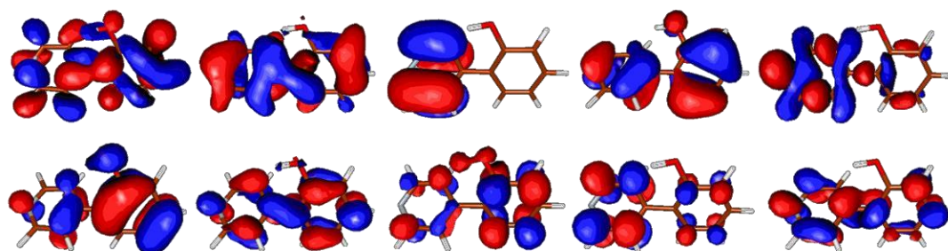
Fig. S2: Canonical molecular orbitals used for the active space of OM2/MRCI method. See main text for details.
