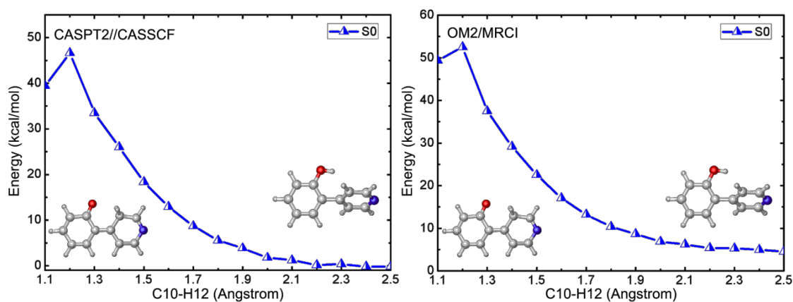
Fig. S3: CASPT2//CASSCF and OM2/MRCI computed S 0 relaxed minimum-energy intramolecular proton transfer path
