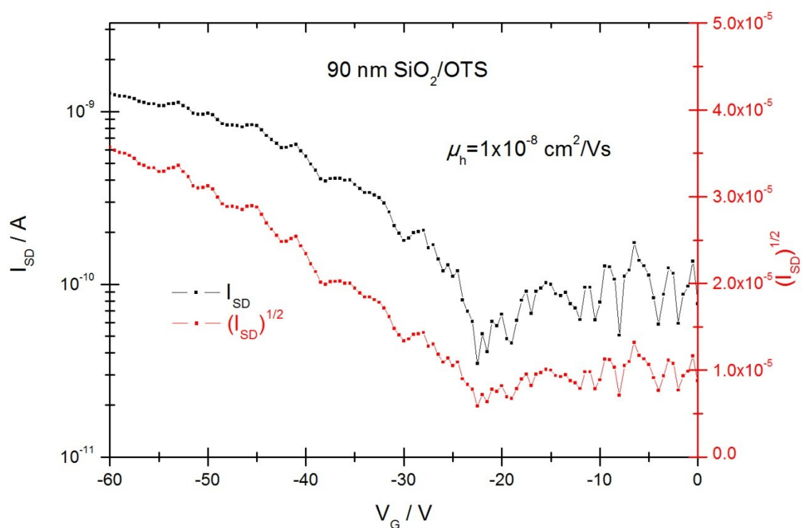
Transfer curve for ethylhexyl N-substituted DPP-based solution processed OFET
