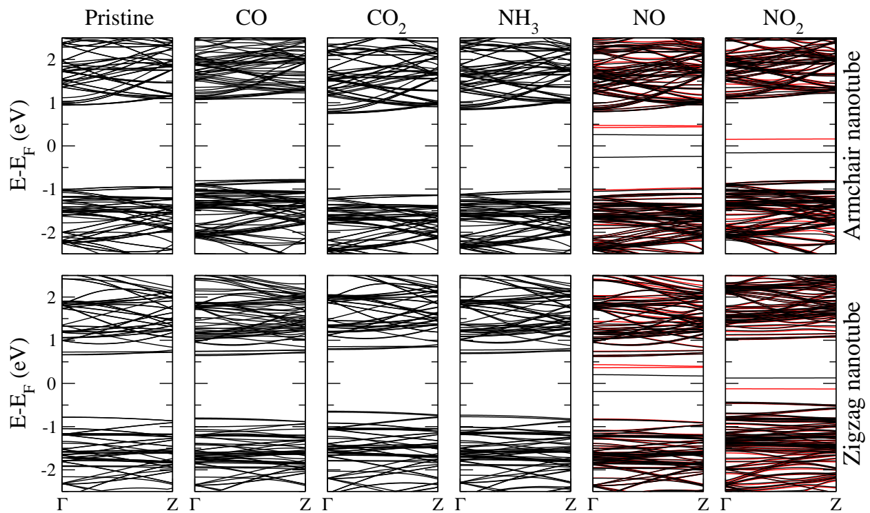
FIG. 1. Band structures corresponding to the densities of states shown in Fig. 3 of the main article.
