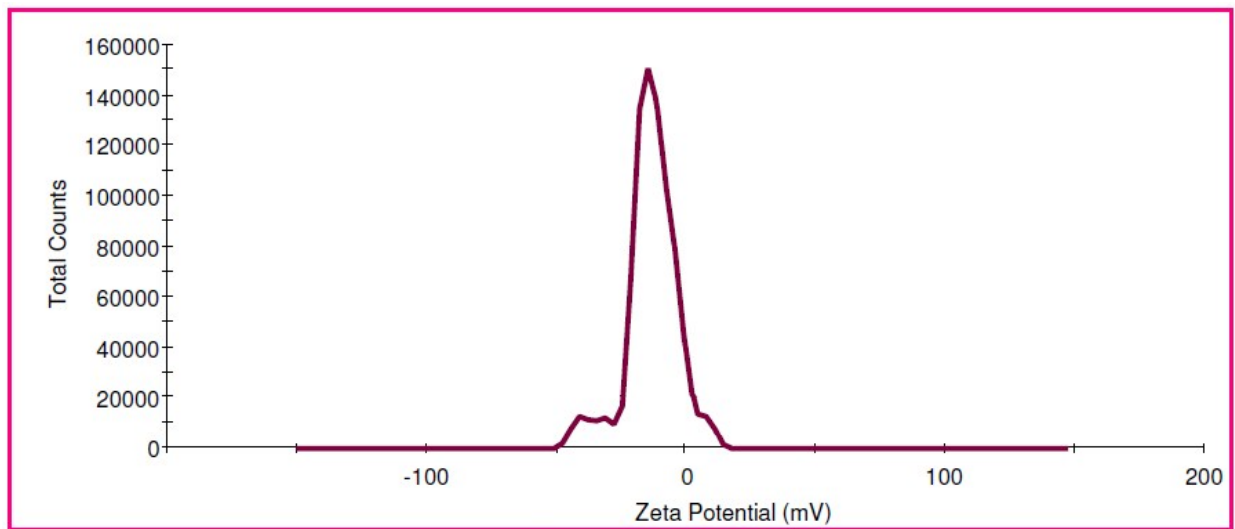
Fig. S2. Zeta potential measurement of AgNPRs in the presence of \text{ClO}^- .
