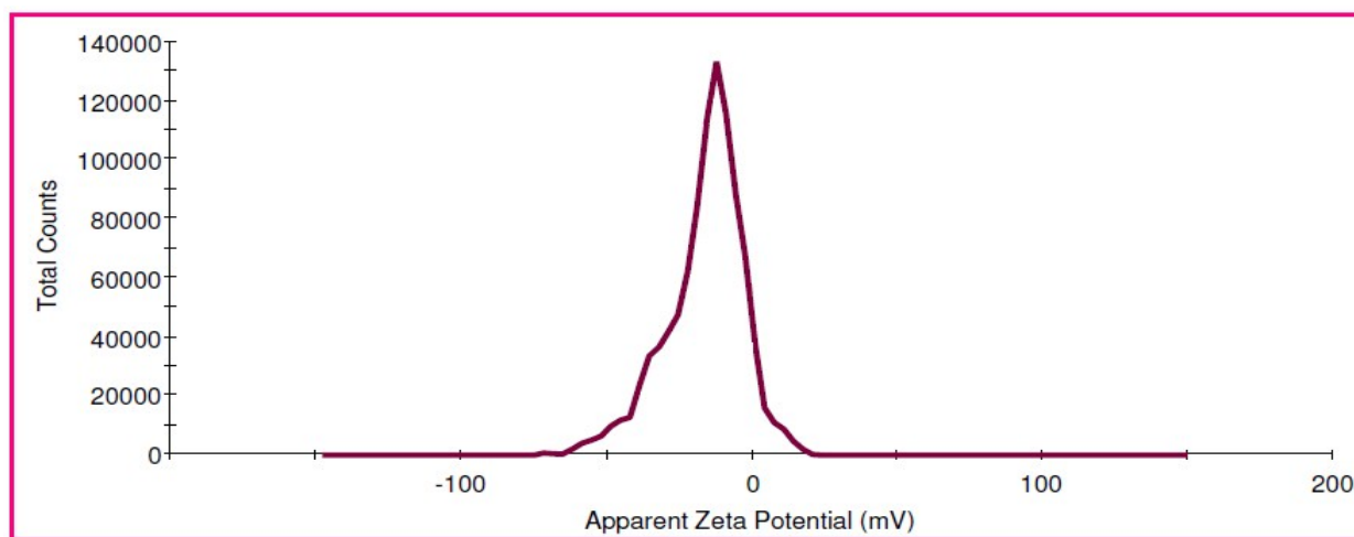
Fig. S1. Zeta potential measurement of AgNPRs.
