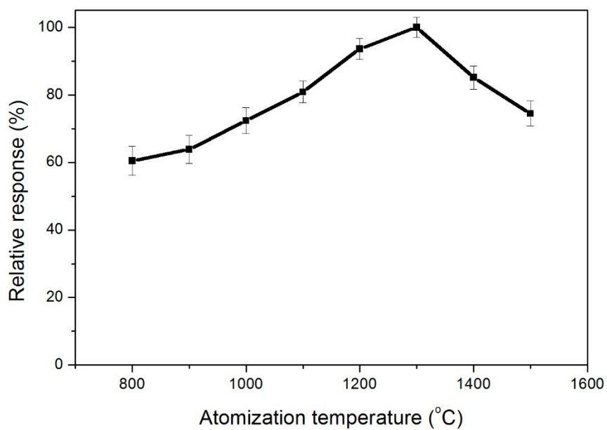
Fig. 2S. Effect of atomization temperature on the analytical response. Other conditions were as indicated in Table 1.
