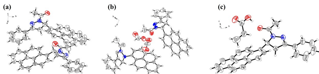
Figure S1. The ORTEP plots of the \beta polymorph (a), the formic acid (b) and propanoic acid (c) solvates.
