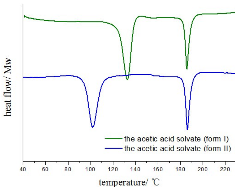
Figure S3. DSC profiles of the acetic acid solvates of APPP (forms I and II).
