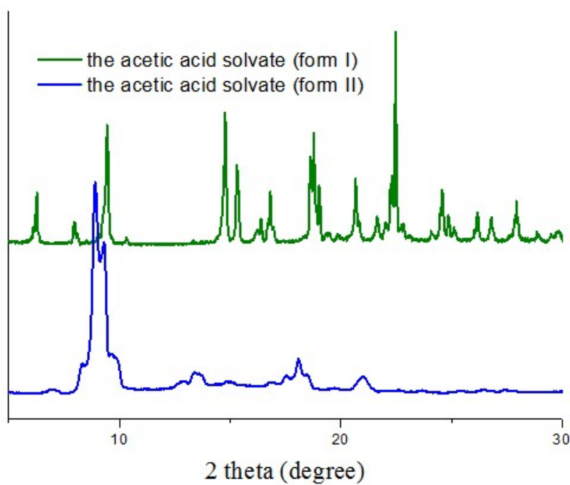
Figure S2. PXRD patterns of the acetic acid solvates of APPP (forms I and II).
