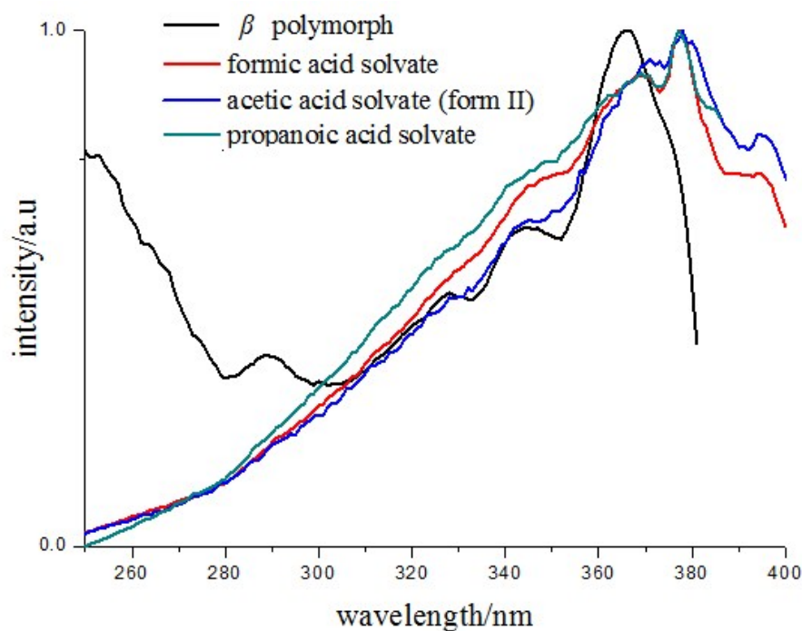
Figure S4. Excitation spectra for these crystals.
