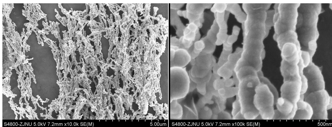
Fig. S2 SEM images of Fe nanofibers formed at [\text{Fe}^{2+}] = 0.2\text{M} .
