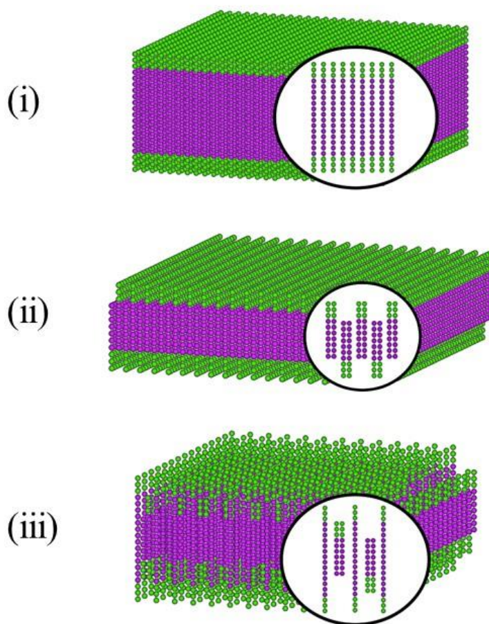
Figure S1. The initial configurations of the membranes formed by A_3B_{14}A_3 triblock copolymers are shown : (i) for I-shaped monolayer membrane, (ii) for U-shaped bilayer membrane, and (iii) for mixed I-shaped/U-shaped membranes.
