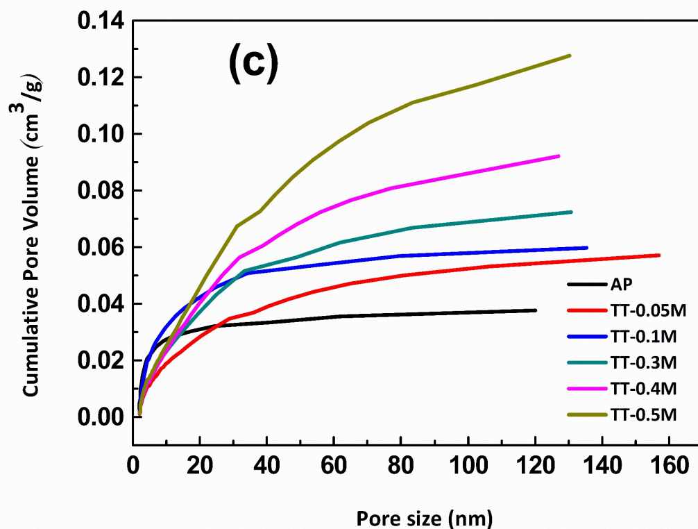
Figure S1. Pore size distribution of as prepared and TPAOH treated samples (a) H-K differential Pore Volume Plot, (b) H-K cumulative pore volume and (c) BJH cumulative pore volume
