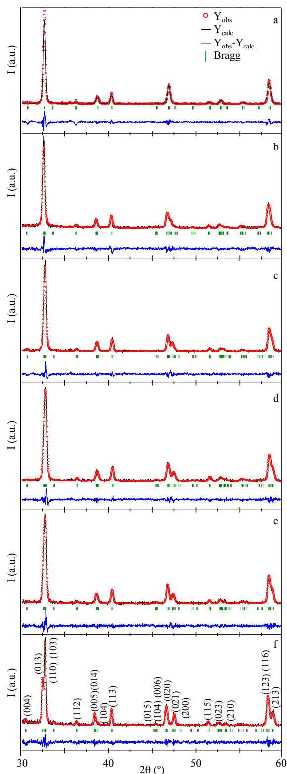
Figure S1. X-ray diffraction patterns of Y100 (a), Y150 (b) Y205 (c), Y250 (d), Y300 (e) and Y500 (f) samples. The calculated patterns obtained from profile refinement of the experimental one together with the difference between both, and the Bragg positions are also depicted.
