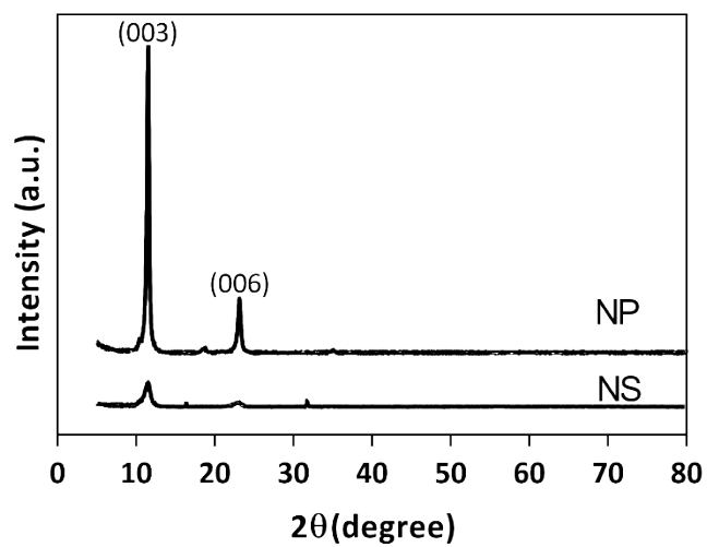
Fig. S1. XRD patterns of LDH NPs and LDH NSs.
