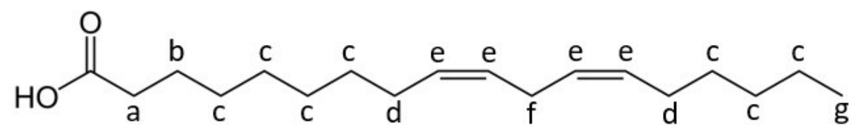
Linoleic acid structure
