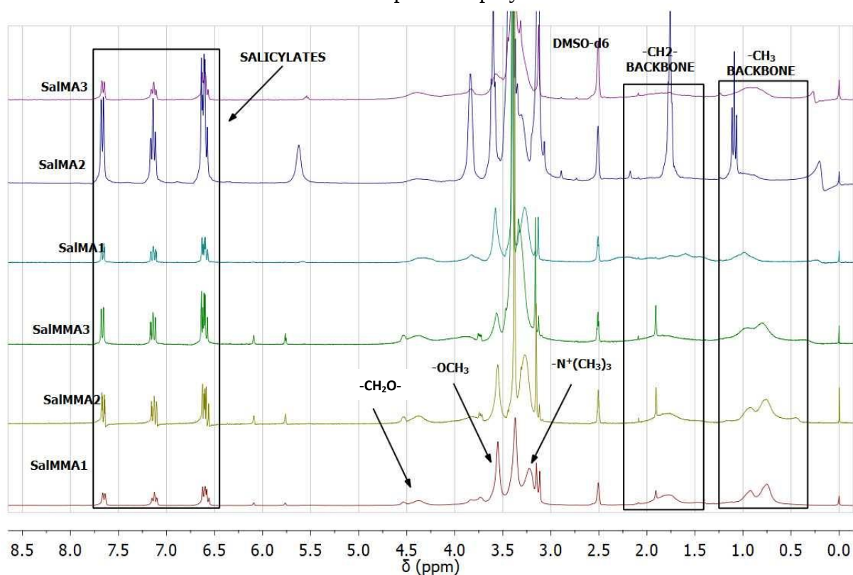
1 H NMR spectra of polymers
