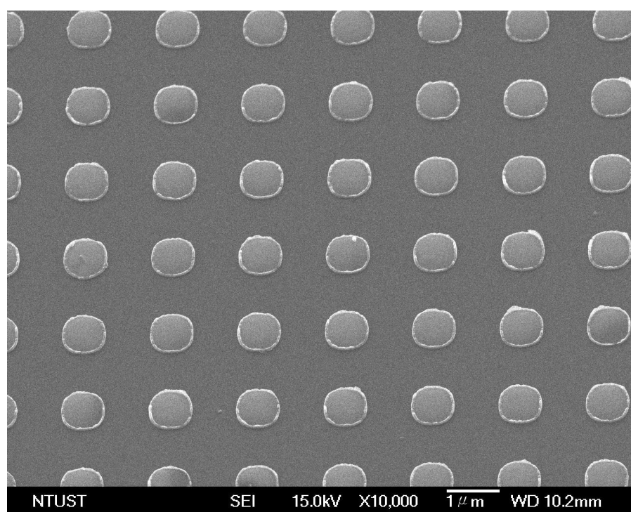
Figure S1 Top-view and titled SEM images of MGNT arrays, deposited for 1125 s, after removal of the photoresist template through ultrasonic cleaning for (a) 45 and (b) 60 sec.
