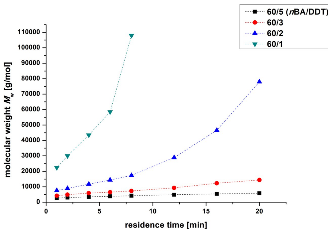
Figure S1: Time dependent M_w development of branched PnBA synthesized in a photo-flow reactor with different monomer-thiol ratios.
