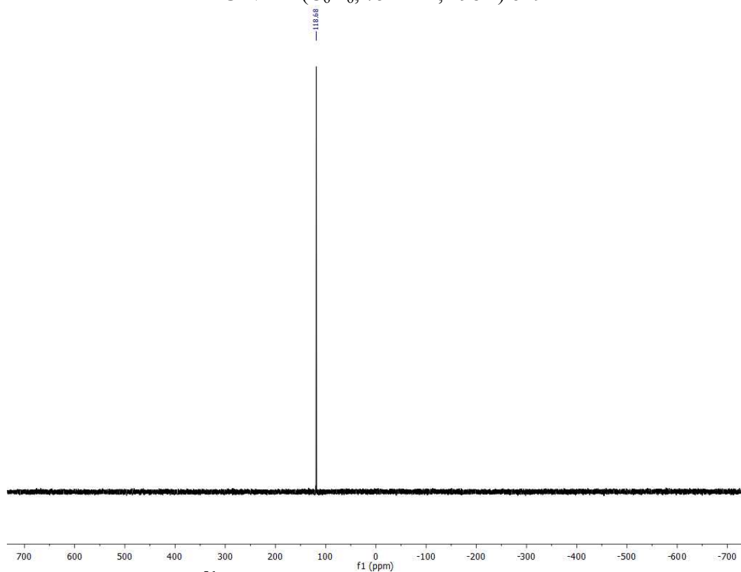
^{31}\text{P} NMR ( \text{C}_6\text{D}_6 , 121 MHz, 298K) of 9
