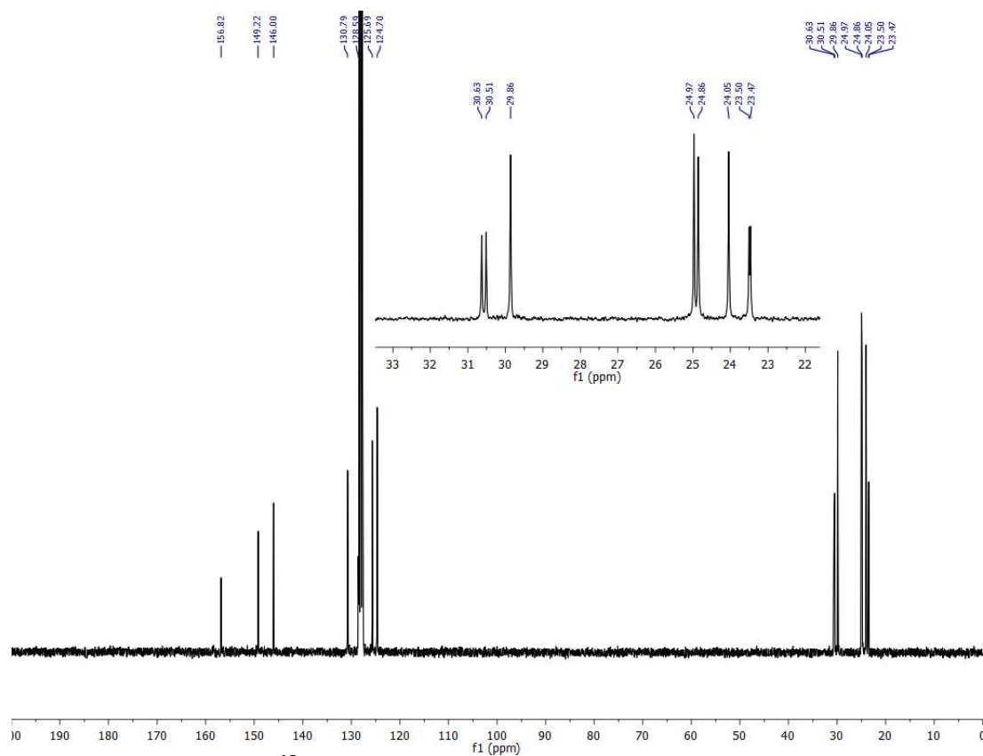
^{13}\text{C} NMR ( \text{C}_6\text{D}_6 , 75 MHz, 298K) of 9
