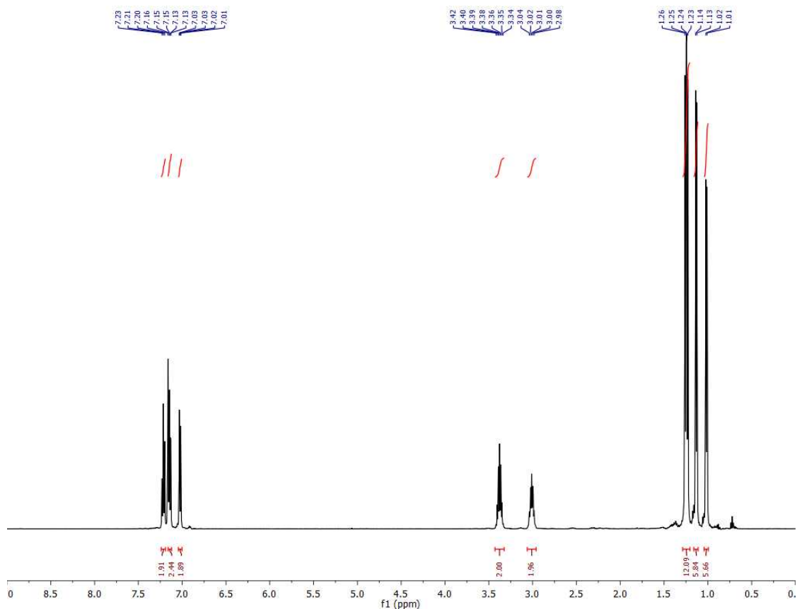
1 H NMR (C 6 D 6 , 300 MHz, 298K) of 9
