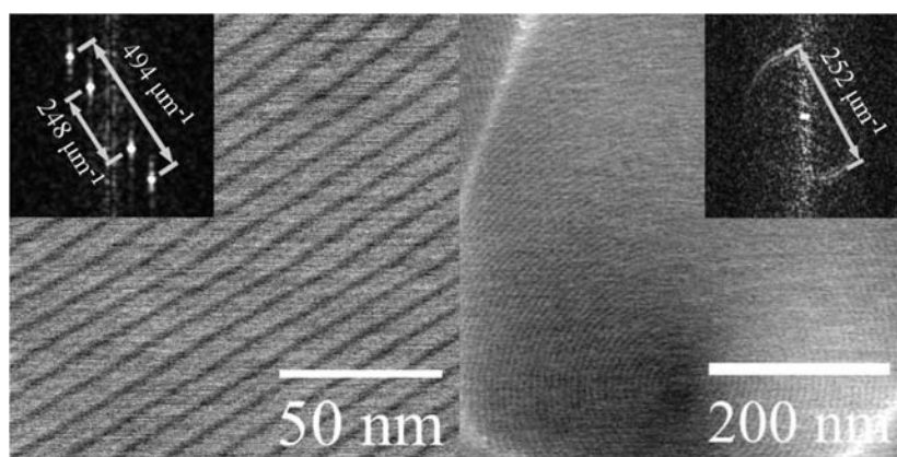
Fig. S14. AFM images of CB7CB in a crystal (left) and N_{TB} (right) phase and the corresponding fast Fourier transform patterns. In the crystalline phase the intensity of the first and second harmonic of the detected periodicity (8.06 nm) is of the same order of magnitude. In the N_{TB} phase only a weak first harmonic (7.93 nm) is detected.
