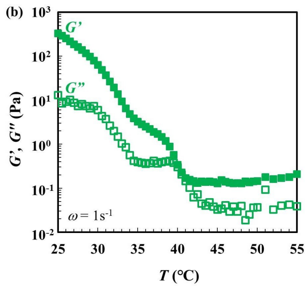
Supporting Information 3. T -dependence of G' and G'' for the suspensions of (a) X_N = 0.8 , \phi_{25} = 1.2 and (b) X_N = 0.7 , \phi_{25} = 1.0 .
