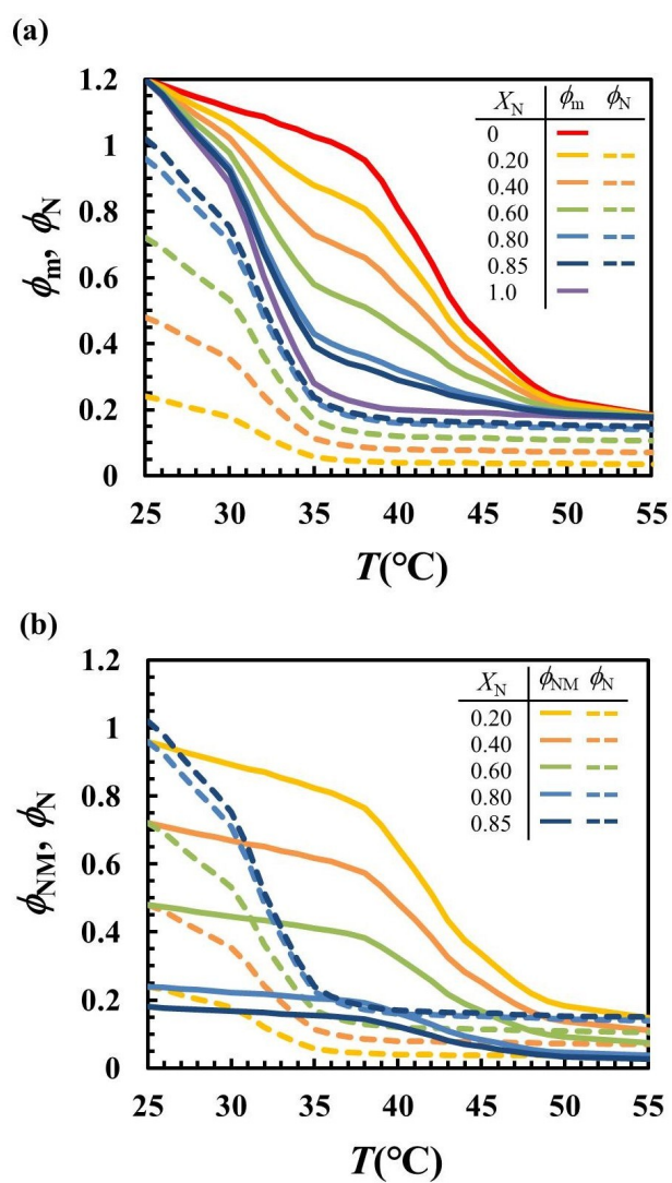
Supporting Information 1. T -dependence of (a) \phi_m and \phi_N , (b) \phi_{NM} and \phi_N for the suspensions of \phi_{25} = 1.2 with various X_N values.
