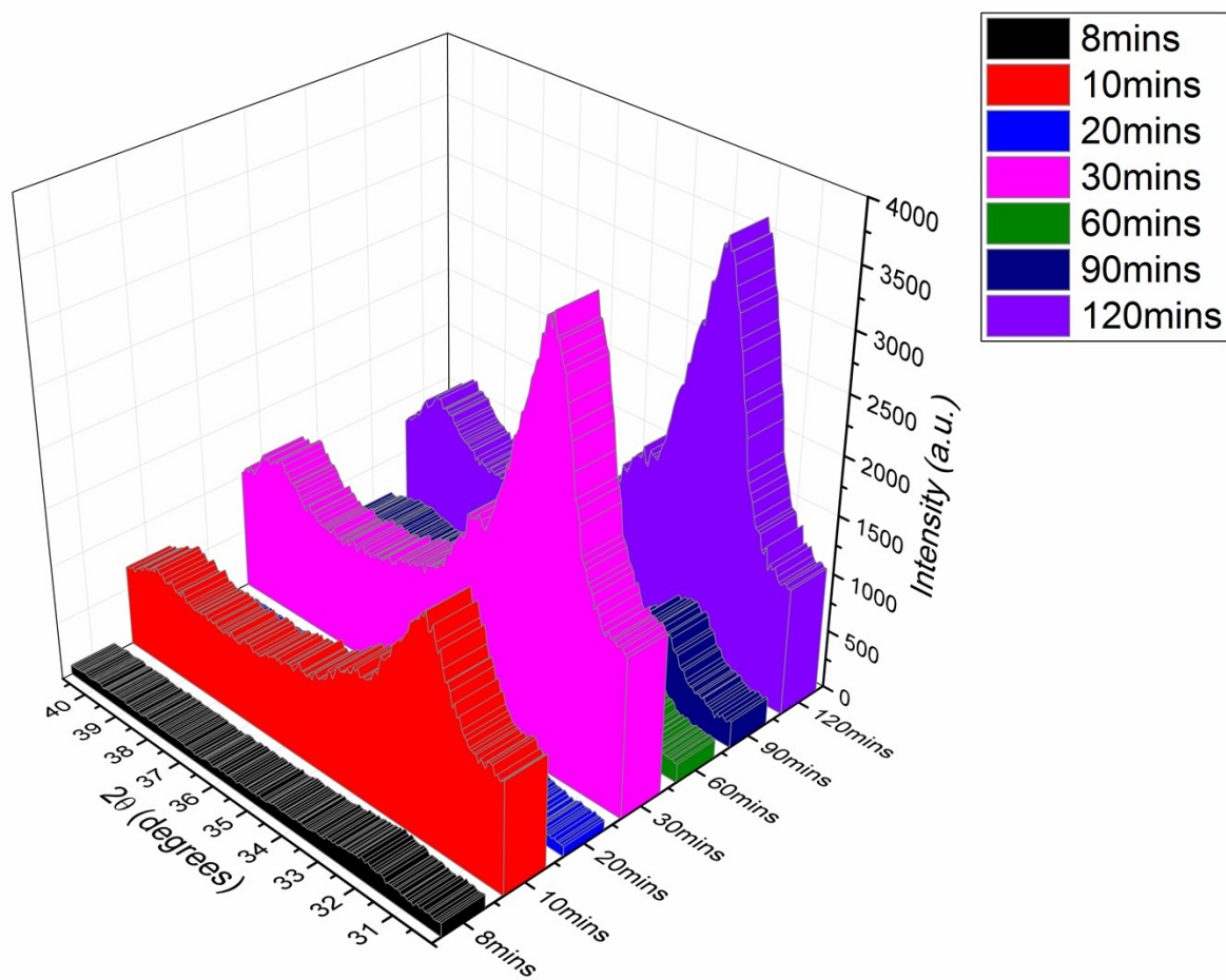
Fig.S1. Timelapse XRD patterns of the composite HAp pastes containing 26.5 wt.% of gelatin in the course of an extended setting reaction with a nonlinear, oscillatory dynamics.
