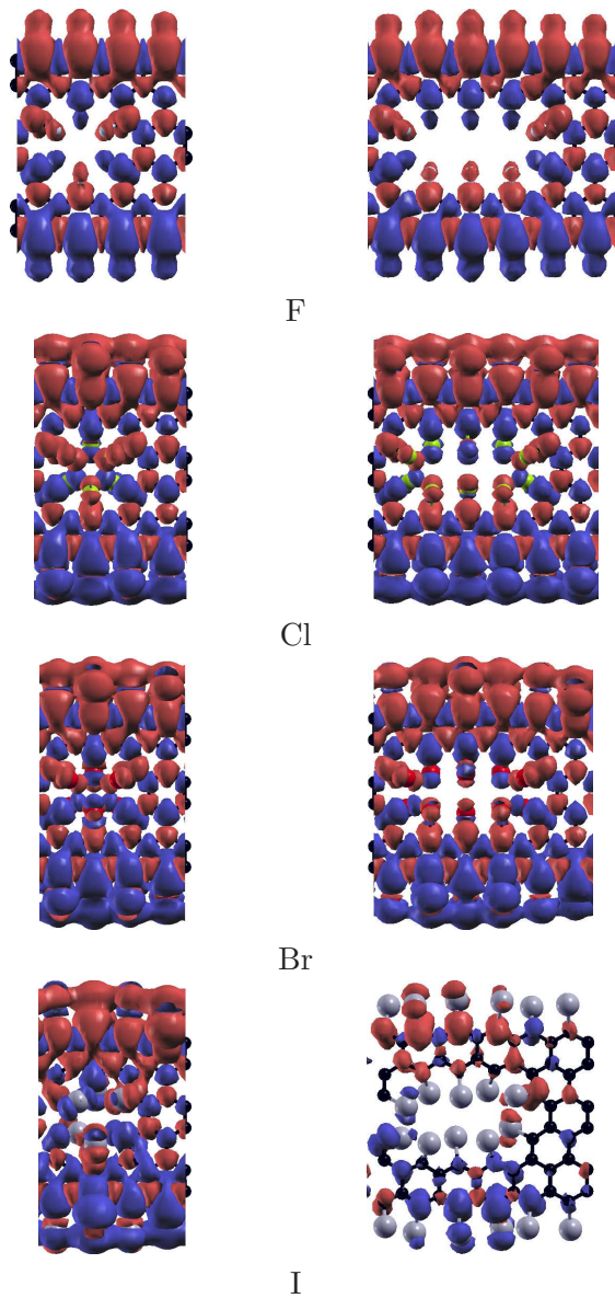
Figure S2: Spin density maps for ZPG1 (left) and ZPG2 (right).
