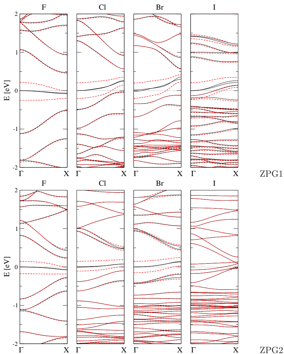
Figure S1: Electronic band structures of ZPG1 and ZPG2: spin unpolarized (black/solid) vs. spin polarized (red/dashed) calculations.
