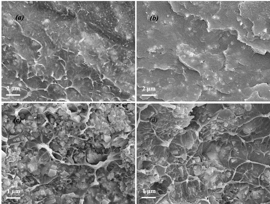
Fig. S1 SEM images of the fractured cross-section of (a) 5 vol% NC-KTN/PVDF composite film, (b) 5 vol% NR-KTN/PVDF composite film, (c) 30 vol% NC-KTN/PVDF composite film and (d) 30 vol% NR-KTN/PVDF composite film.
