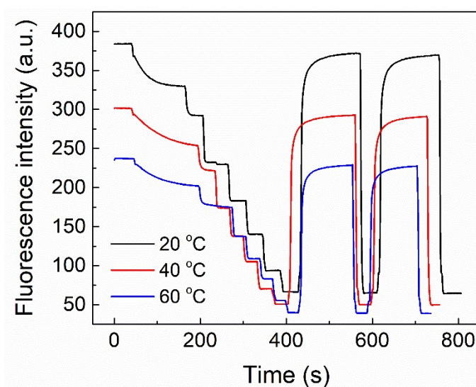
Fig. S2 The response of oxygen sensor in different concentrations of oxygen at three different temperatures.
