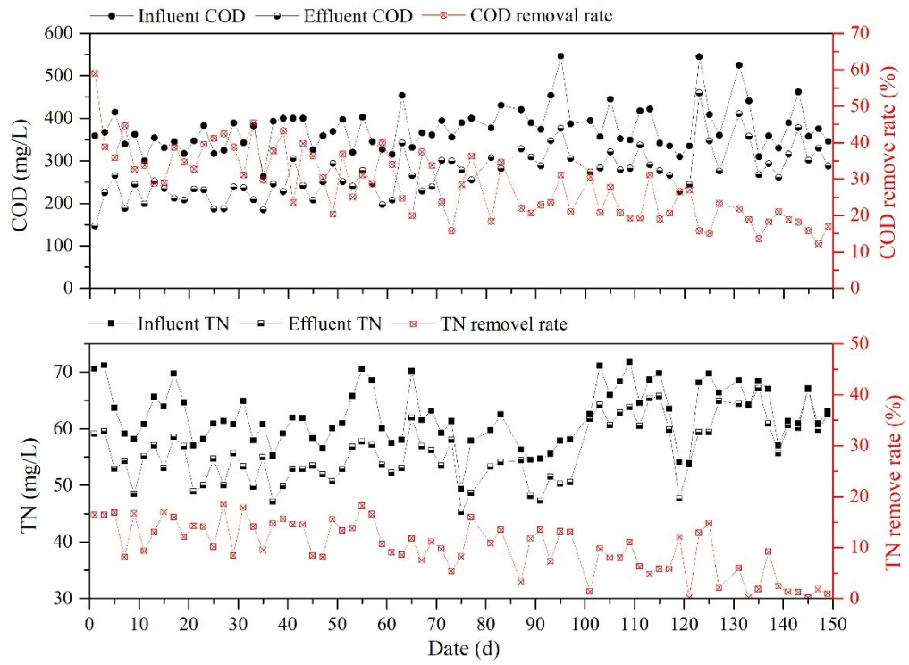
Figure S2. Performance of SBR2 under different dissolved oxygen concentrations.
