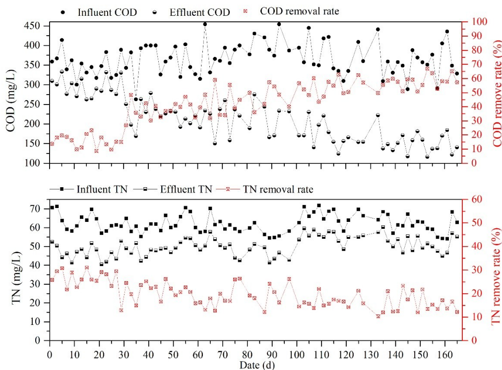
Figure S1. Performance of SBR1 under different dissolved oxygen concentrations.
