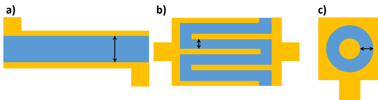
Figure S1. Schematic of the test structures with a) in-plane, b) interdigitated fingers and c) co-centric circular electrodes. The arrow shows the spacing between the electrodes which was varied. The yellow regions indicate the electrode area. The blue region represents graphene oxide.
