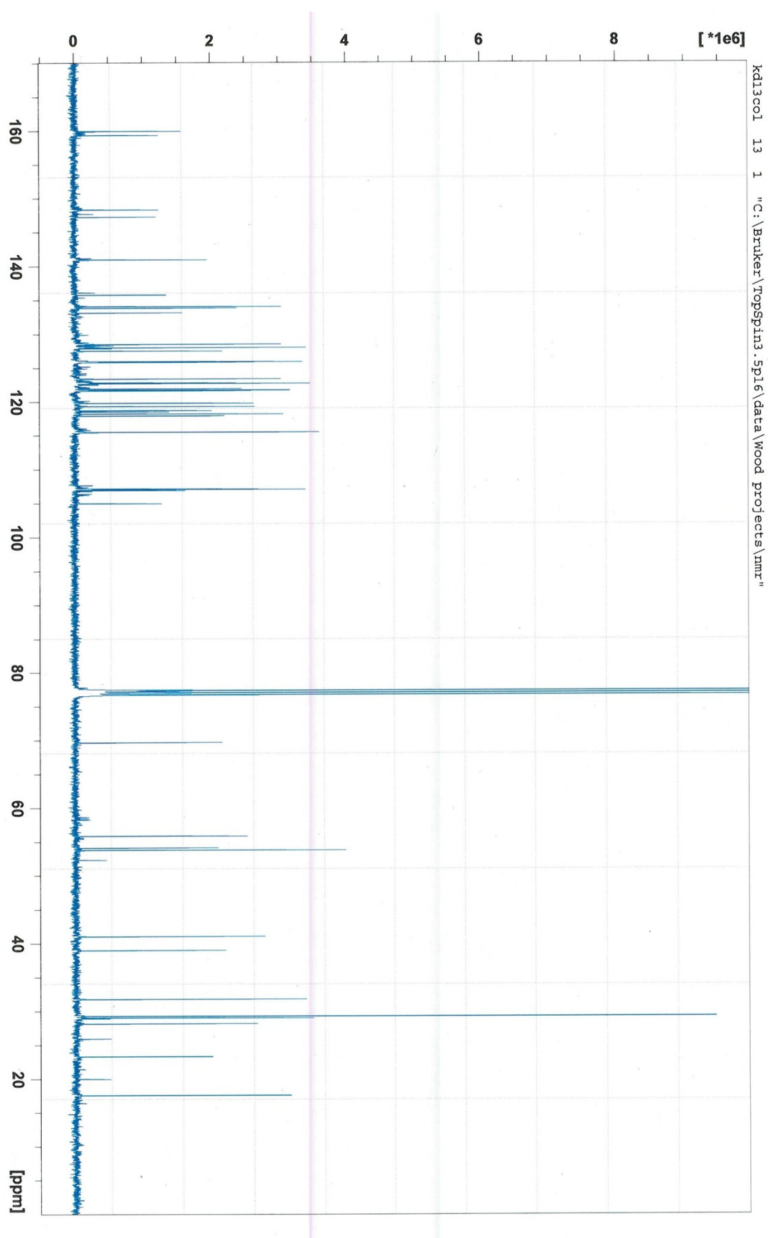
^{13}\text{C} NMR spectrum for 6f
