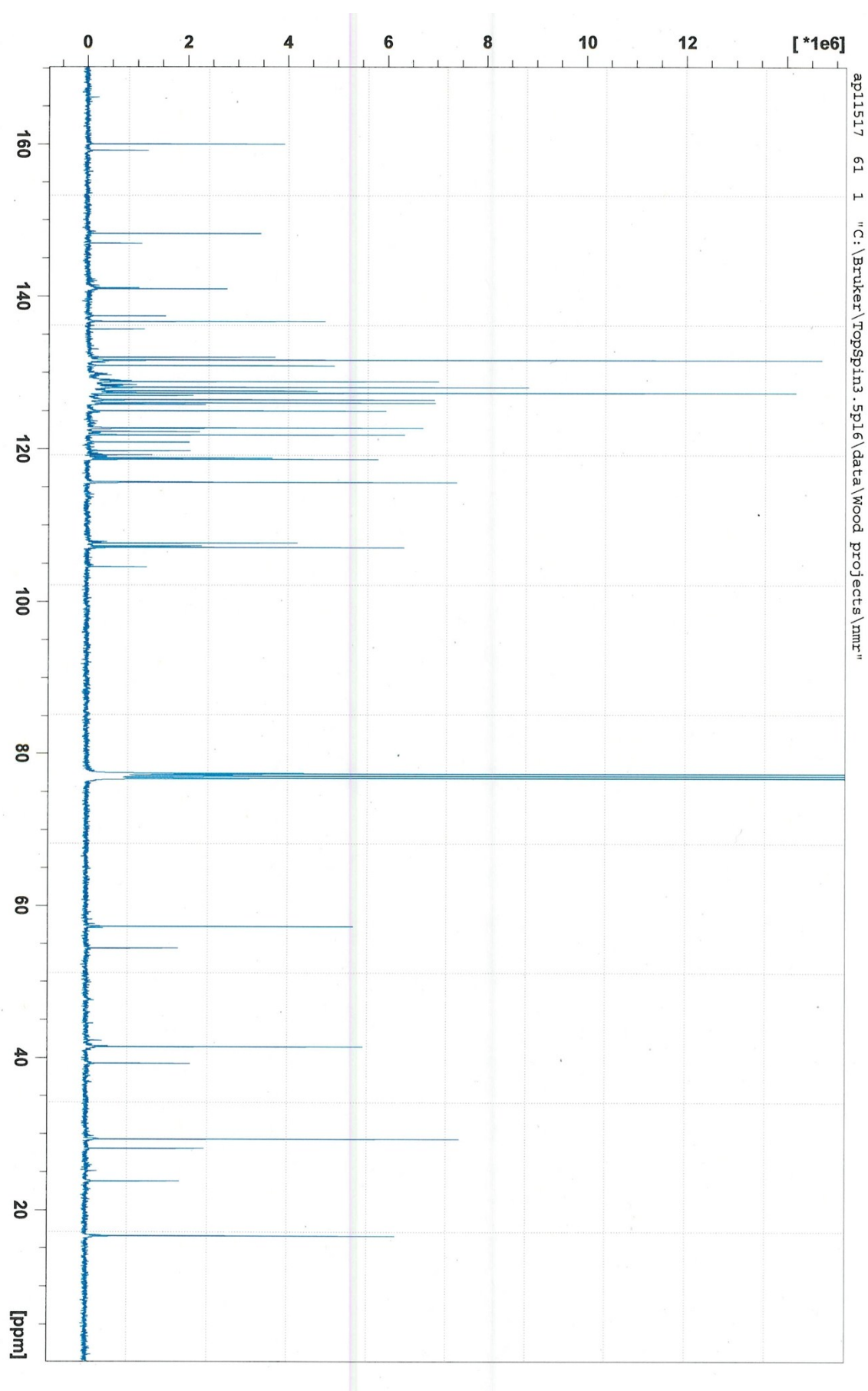
^{13}\text{C} NMR spectrum for 6a
