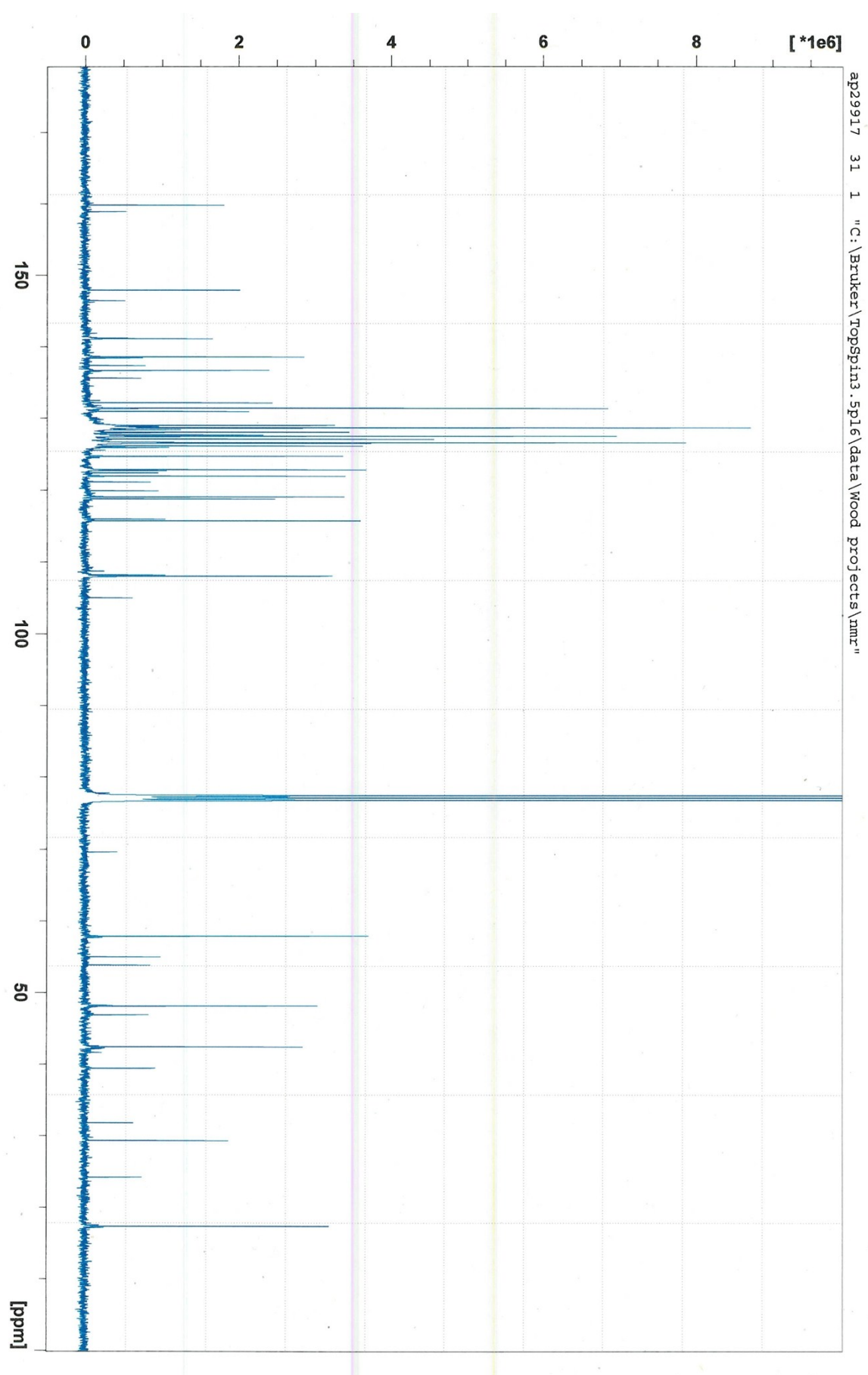
^{13}\text{C} NMR spectrum for 6o
