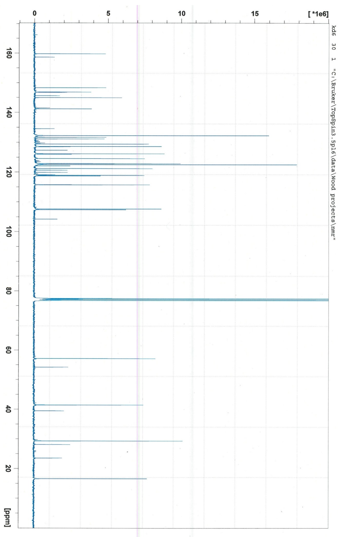
^{13}\text{C} NMR spectrum for 6c
