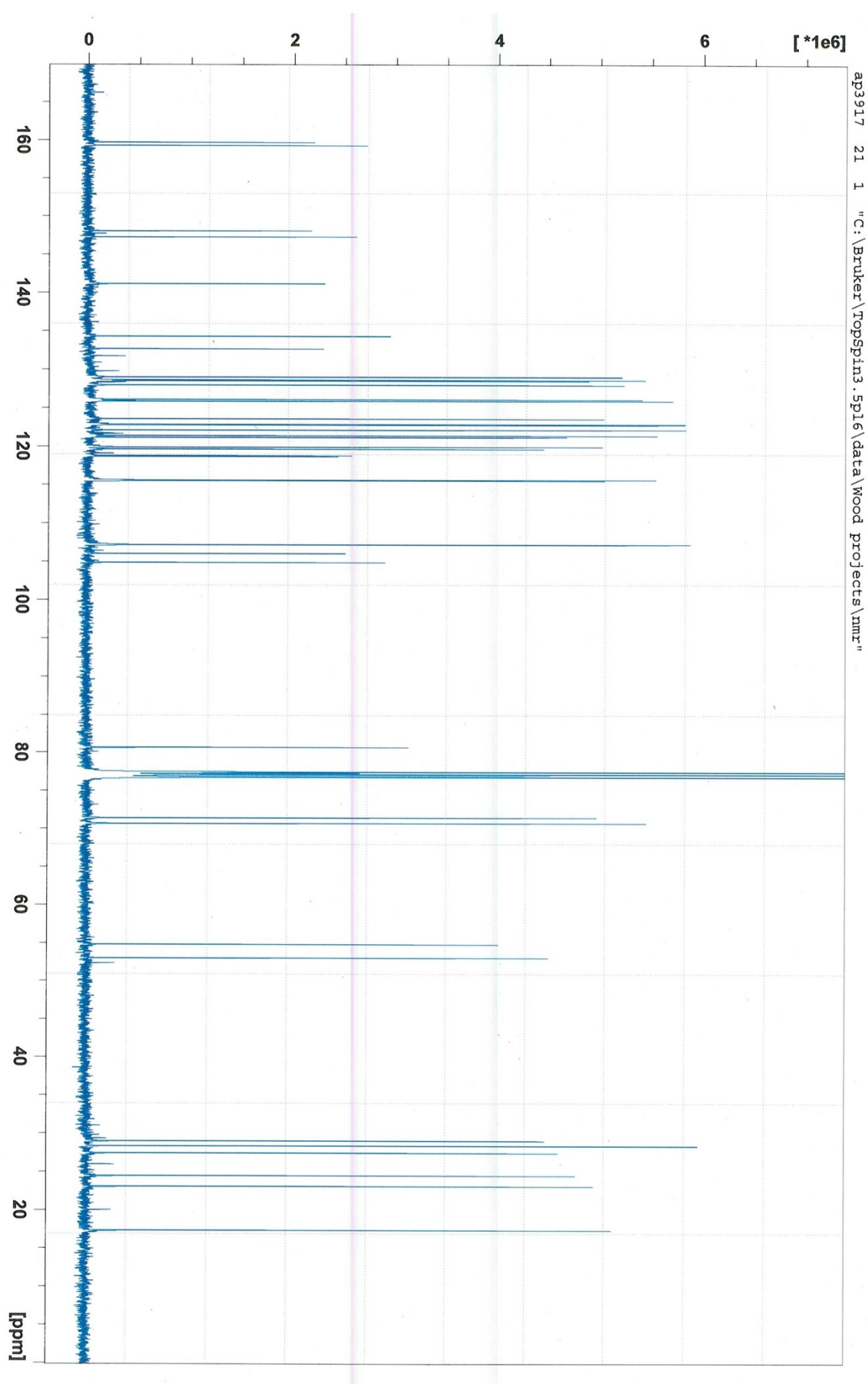
^{13}\text{C} NMR spectrum for 6g
