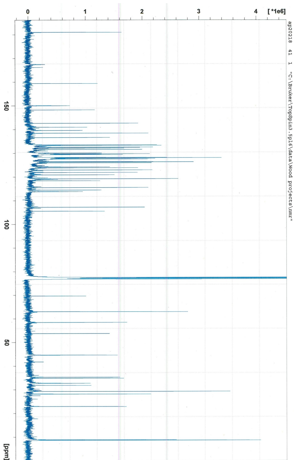
^{13}\text{C} NMR spectrum for 6n
