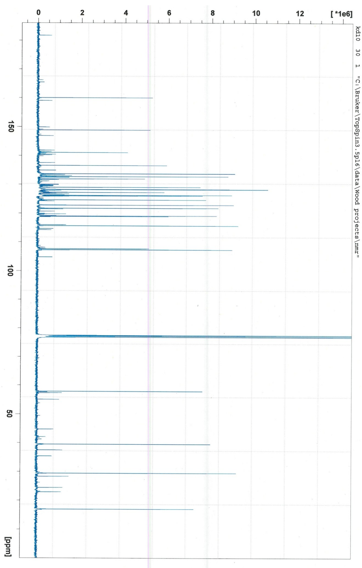
13 C NMR spectrum for 6d
