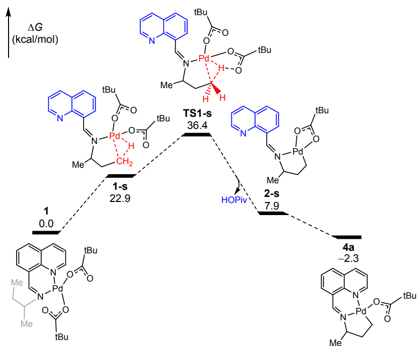
Fig. S1. Free energy profiles for the pivalate-assisted inner-sphere AMLA/CMD C(sp 3 )–H activation without the dissociation of pivalate.
