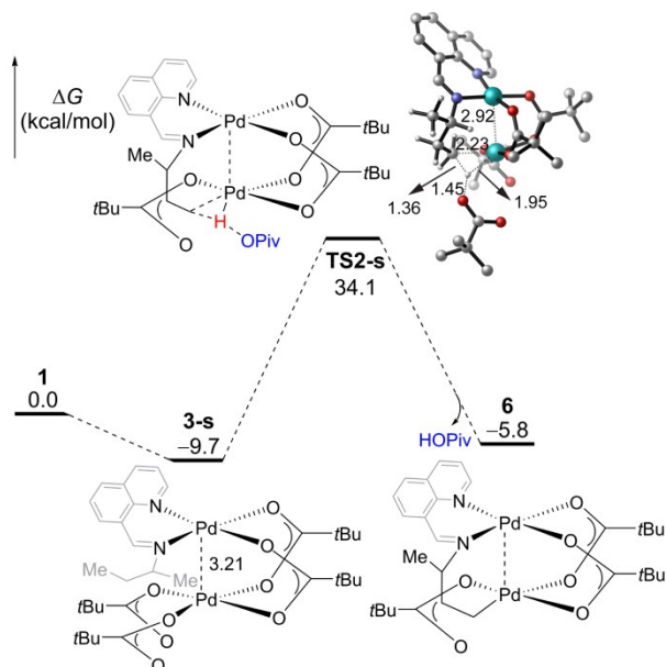
Fig. S2. Free energy profiles for the outer-sphere AMLA/CMD C(sp 3 )–H activation with the binuclear palladium species, and bond lengths are given in Å.
