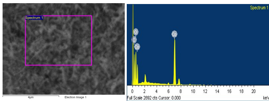
Fig. S3 EDS spectra of the CCNF
