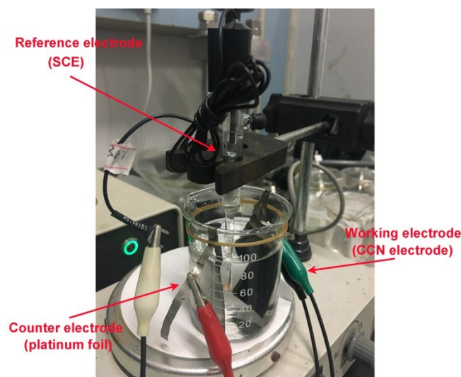
Fig. S2 The configuration of electrochemical tests.
