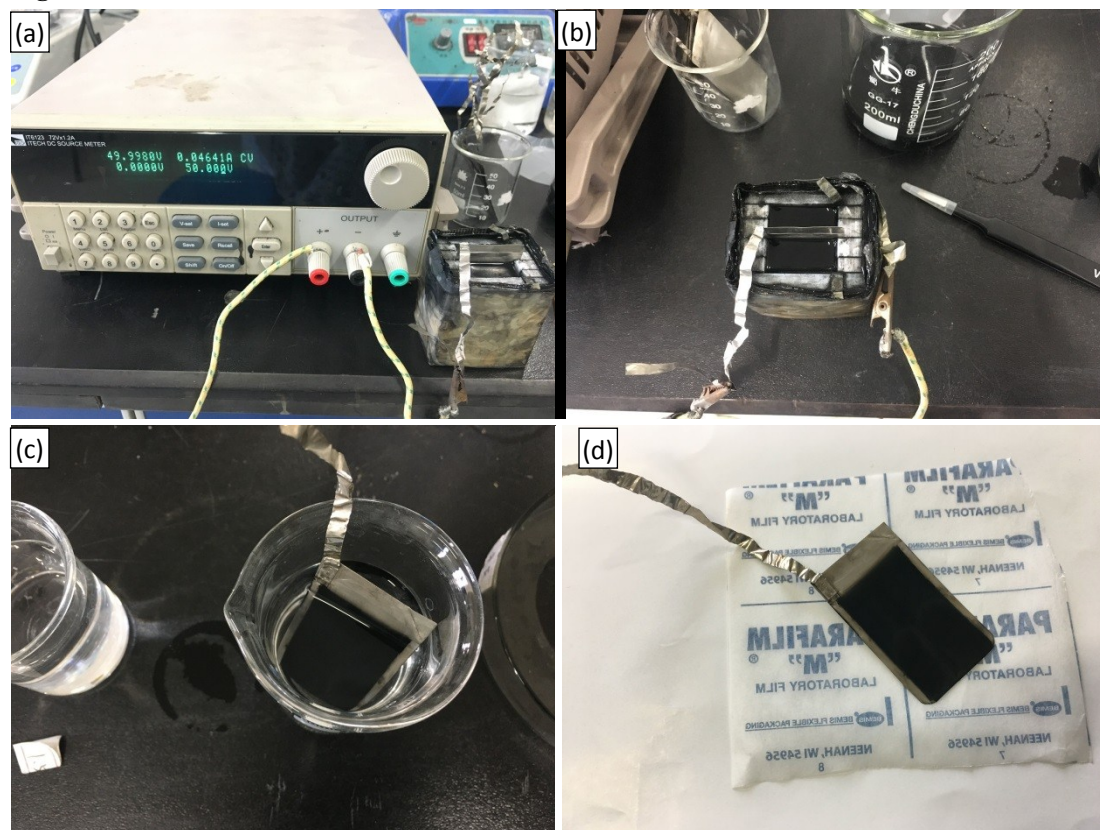
Fig. S1 The photos of the experimental setup and CCNF electrode sample: (a) Experimental setup, (b) Electrolytic cell, (c) Washing by dipping in absolute ethanol and (d) The CCNF electrode.
